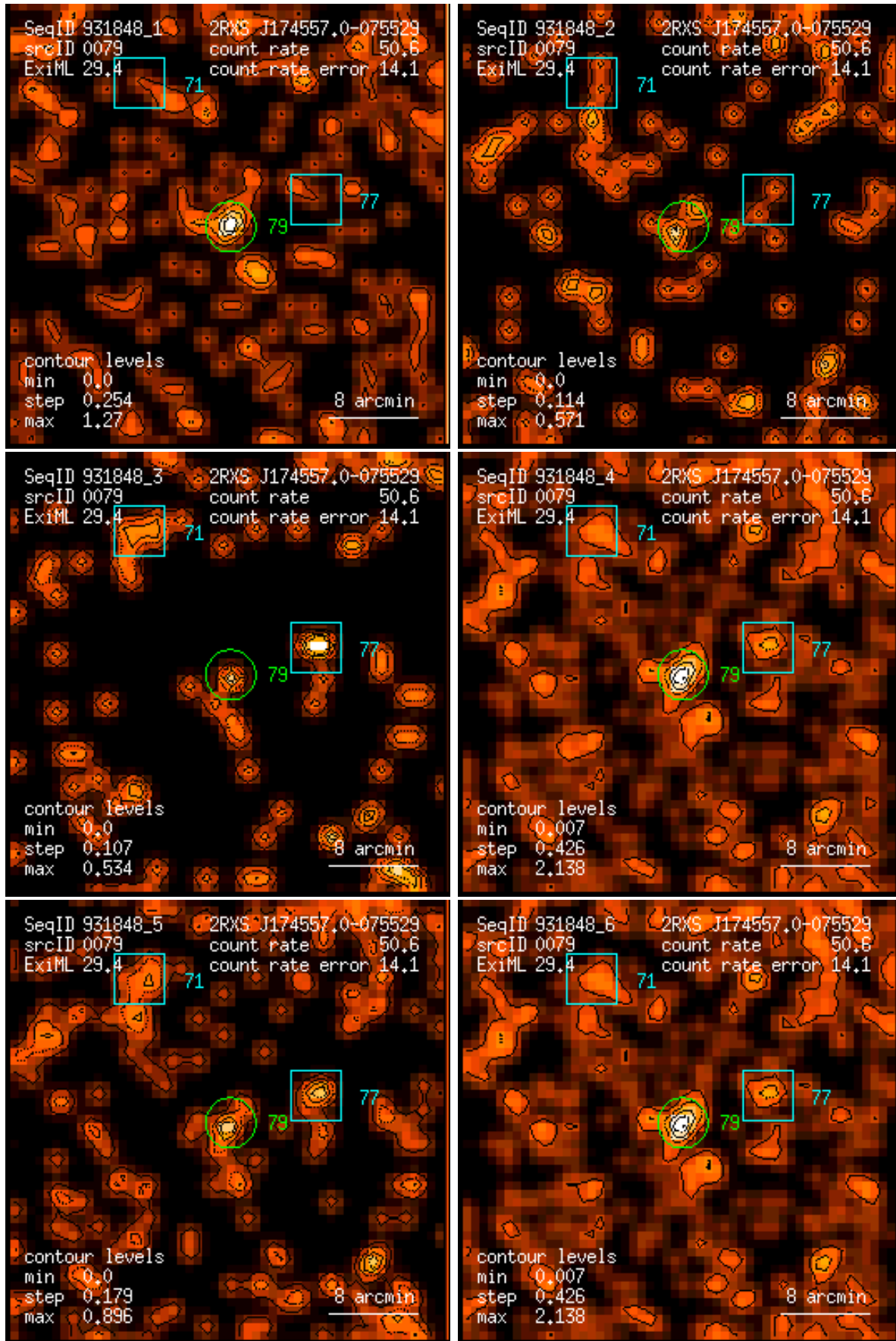
Figure 79: RASS 931848: detection 0079: band rate images, Gaussian filter: (1) PSPC channels 11 – 41, (2) 52 – 90, (3) 91 – 201, (4) 11 – 235, (5) 52 – 201, (6) 11 – 201. Broad band rates in counts/ks. Band rate contour levels in counts/ks/arcmin 2 .
