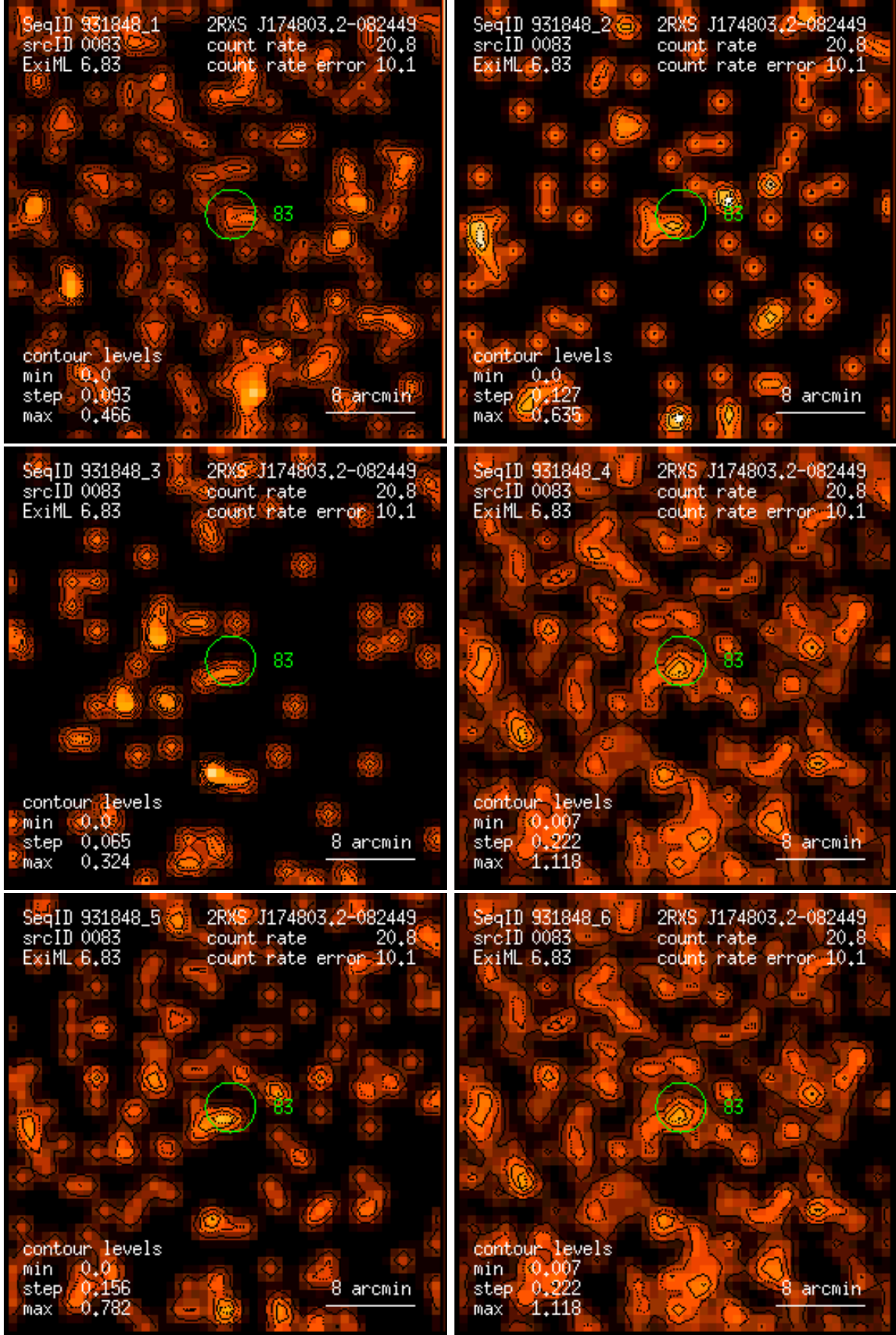
Figure 83: RASS 931848: detection 0083: band rate images, Gaussian filter: (1) PSPC channels 11 – 41, (2) 52 – 90, (3) 91 – 201, (4) 11 – 235, (5) 52 – 201, (6) 11 – 201. Broad band rates in counts/ks. Band rate contour levels in counts/ks/arcmin 2 .
