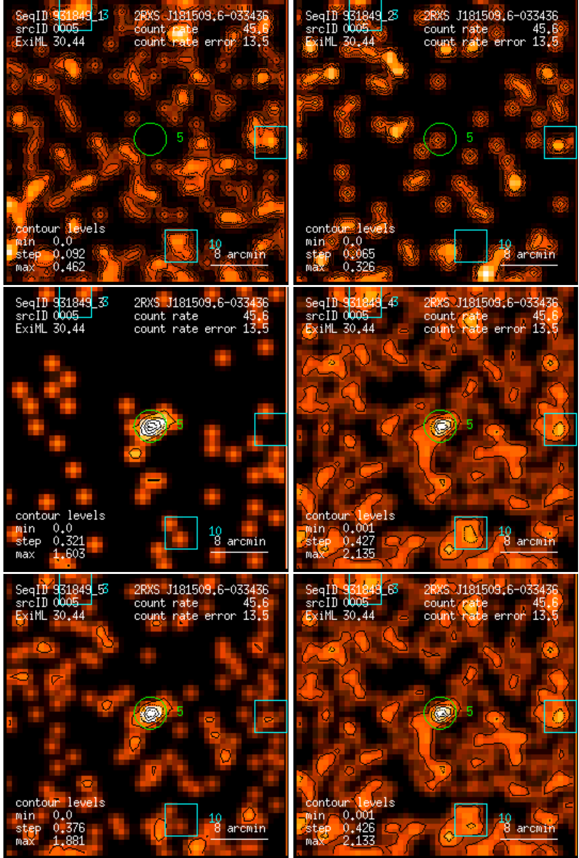
Figure 5: RASS 931849: detection 0005: band rate images, Gaussian filter: (1) PSPC channels 11 – 41, (2) 52 – 90, (3) 91 – 201, (4) 11 – 235, (5) 52 – 201, (6) 11 – 201. Broad band rates in counts/ks. Band rate contour levels in counts/ks/arcmin 2 .
