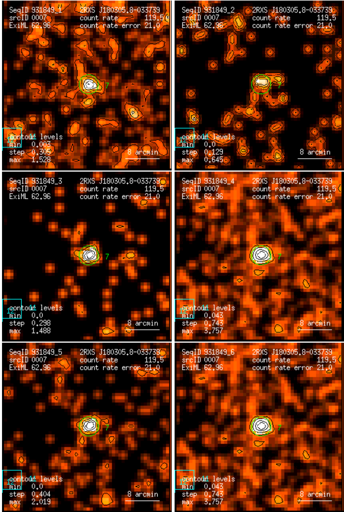
Figure 7: RASS 931849: detection 0007: band rate images, Gaussian filter: (1) PSPC channels 11 – 41, (2) 52 – 90, (3) 91 – 201, (4) 11 – 235, (5) 52 – 201, (6) 11 – 201. Broad band rates in counts/ks. Band rate contour levels in counts/ks/arcmin 2 .
