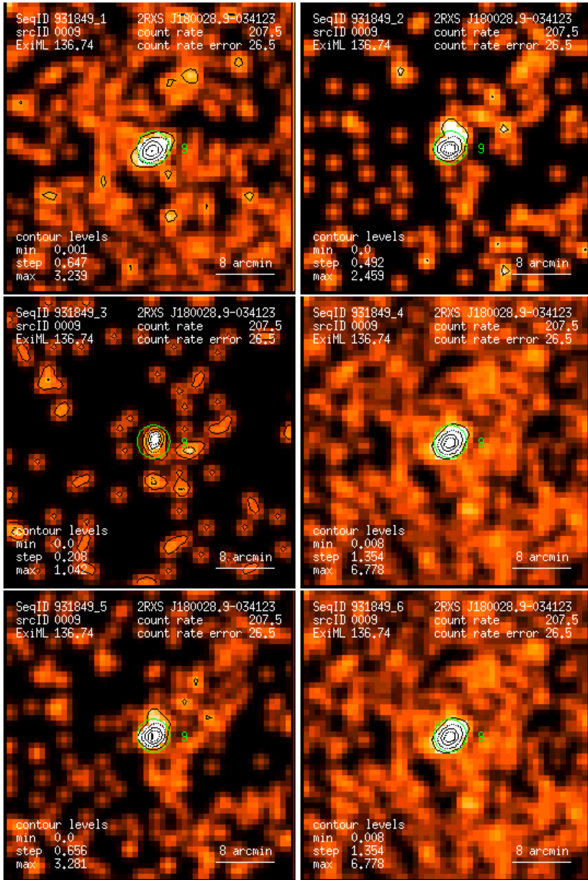
Figure 9: RASS 931849: detection 0009: band rate images, Gaussian filter: (1) PSPC channels 11 – 41, (2) 52 – 90, (3) 91 – 201, (4) 11 – 235, (5) 52 – 201, (6) 11 – 201. Broad band rates in counts/ks. Band rate contour levels in counts/ks/arcmin 2 .
