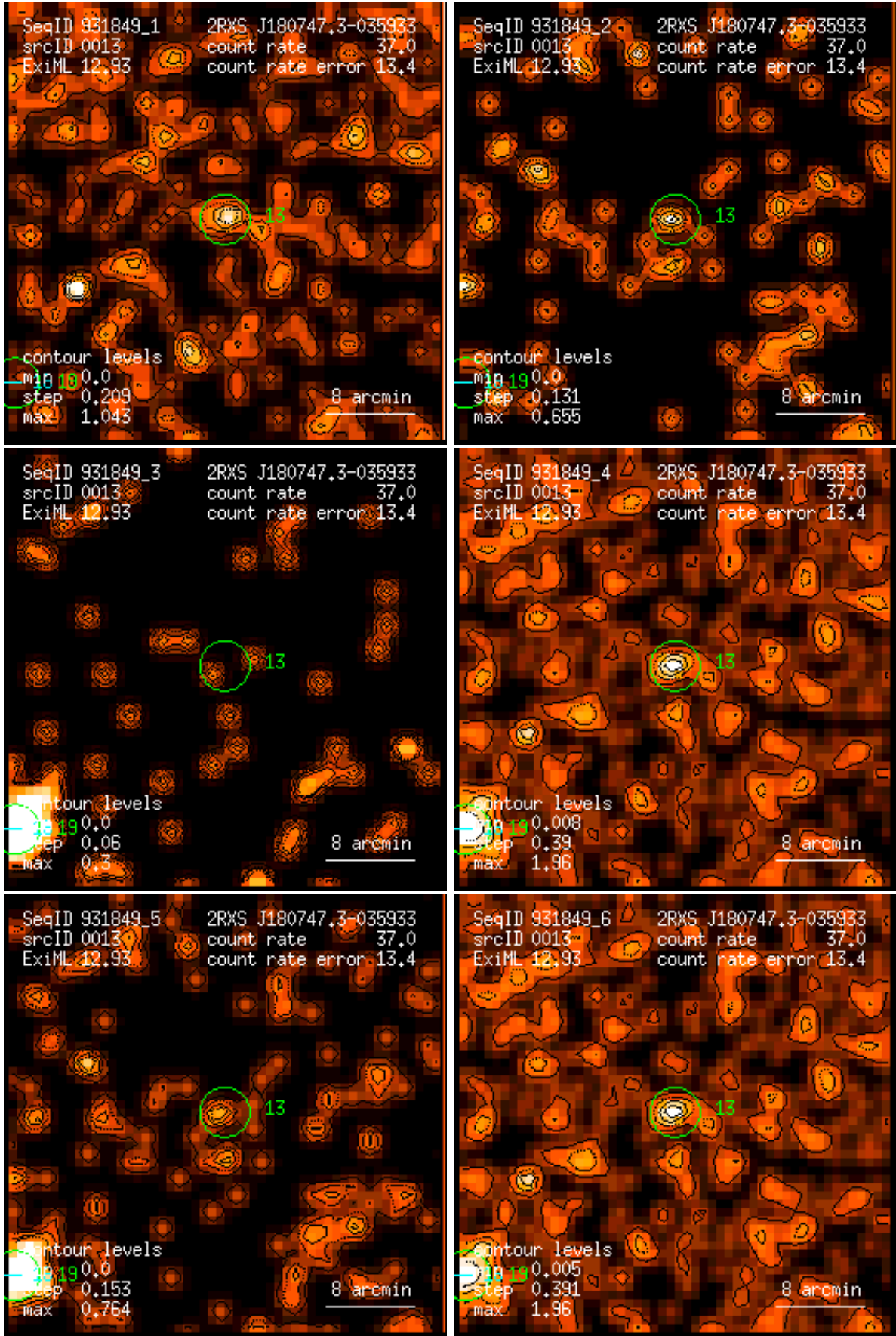
Figure 13: RASS 931849: detection 0013: band rate images, Gaussian filter: (1) PSPC channels 11 – 41, (2) 52 – 90, (3) 91 – 201, (4) 11 – 235, (5) 52 – 201, (6) 11 – 201. Broad band rates in counts/ks. Band rate contour levels in counts/ks/arcmin 2 .
