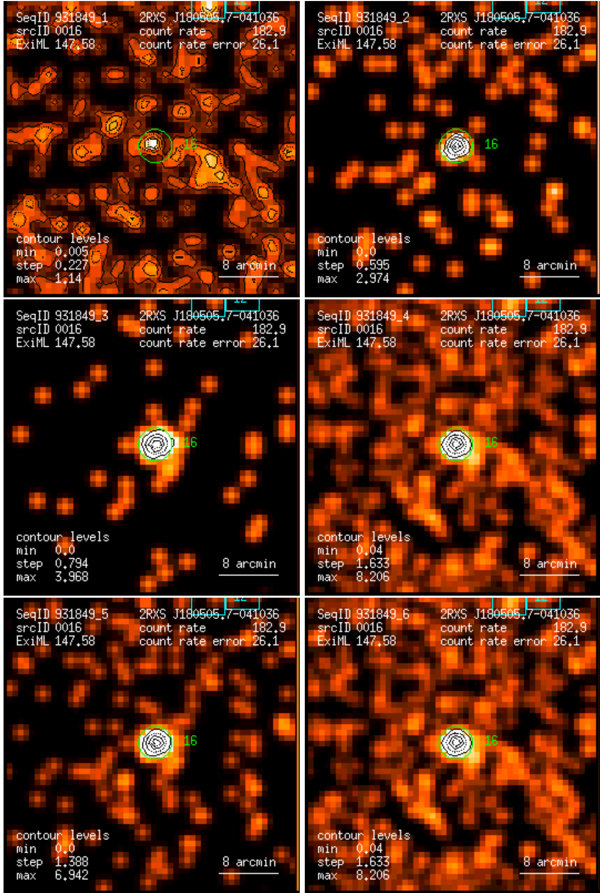
Figure 16: RASS 931849: detection 0016: band rate images, Gaussian filter: (1) PSPC channels 11 – 41, (2) 52 – 90, (3) 91 – 201, (4) 11 – 235, (5) 52 – 201, (6) 11 – 201. Broad band rates in counts/ks. Band rate contour levels in counts/ks/arcmin 2 .
