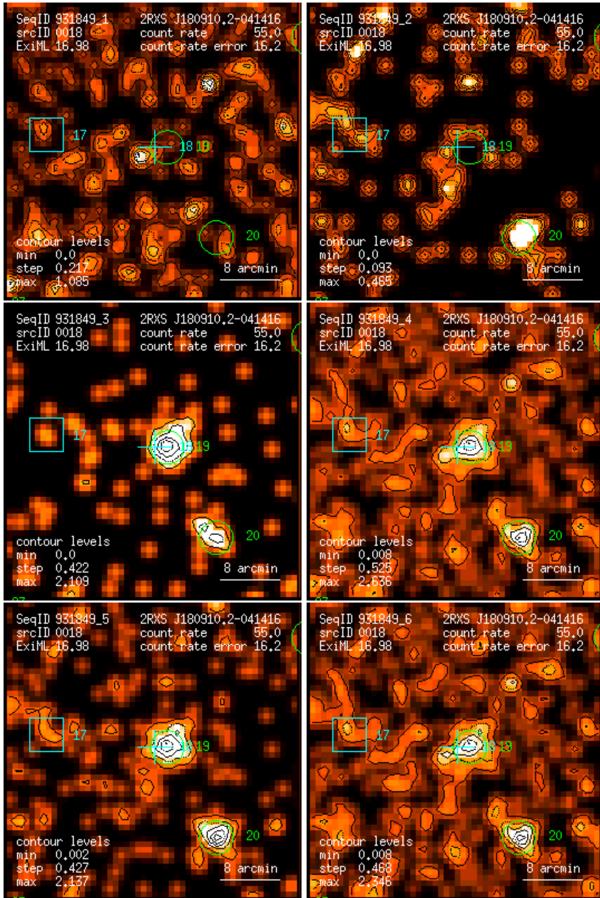
Figure 18: RASS 931849: detection 0018: band rate images, Gaussian filter: (1) PSPC channels 11 – 41, (2) 52 – 90, (3) 91 – 201, (4) 11 – 235, (5) 52 – 201, (6) 11 – 201. Broad band rates in counts/ks. Band rate contour levels in counts/ks/arcmin 2 .
