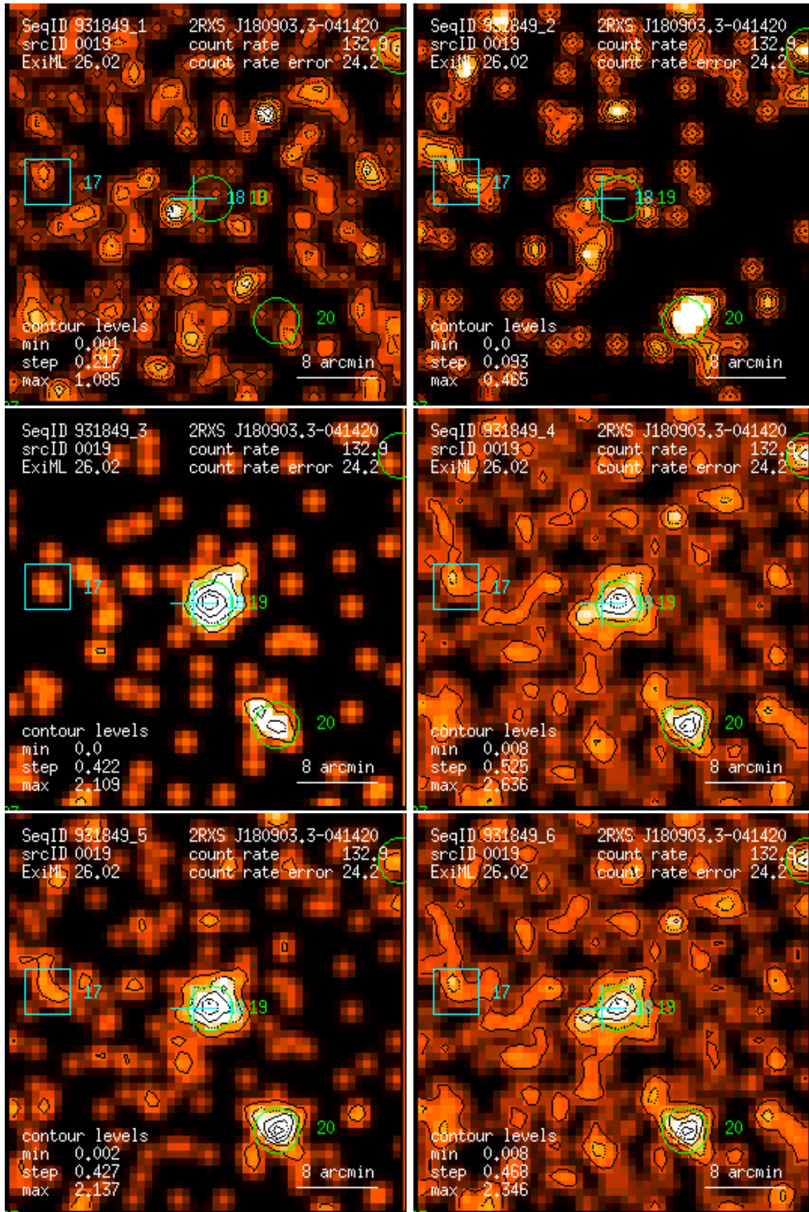
Figure 19: RASS 931849: detection 0019: band rate images, Gaussian filter: (1) PSPC channels 11 – 41, (2) 52 – 90, (3) 91 – 201, (4) 11 – 235, (5) 52 – 201, (6) 11 – 201. Broad band rates in counts/ks. Band rate contour levels in counts/ks/arcmin 2 .
