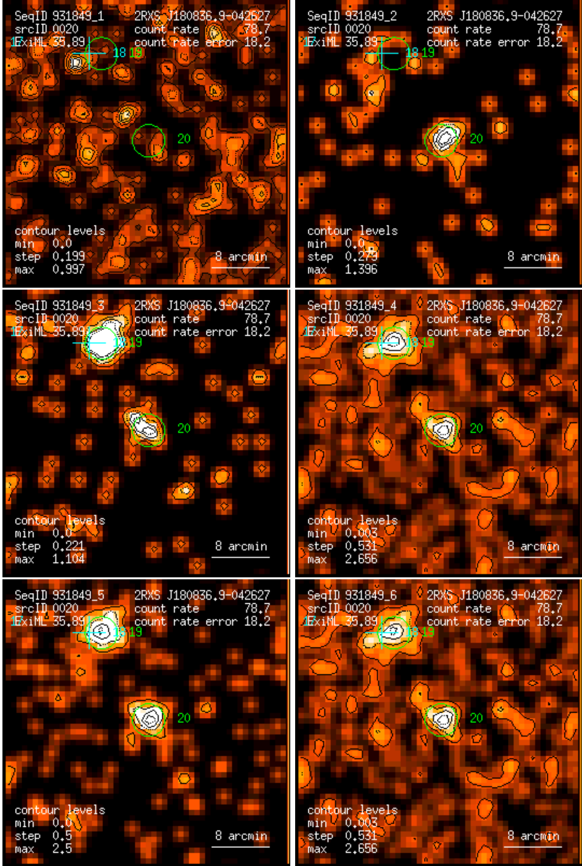
Figure 20: RASS 931849: detection 0020: band rate images, Gaussian filter: (1) PSPC channels 11 – 41, (2) 52 – 90, (3) 91 – 201, (4) 11 – 235, (5) 52 – 201, (6) 11 – 201. Broad band rates in counts/ks. Band rate contour levels in counts/ks/arcmin 2 .
