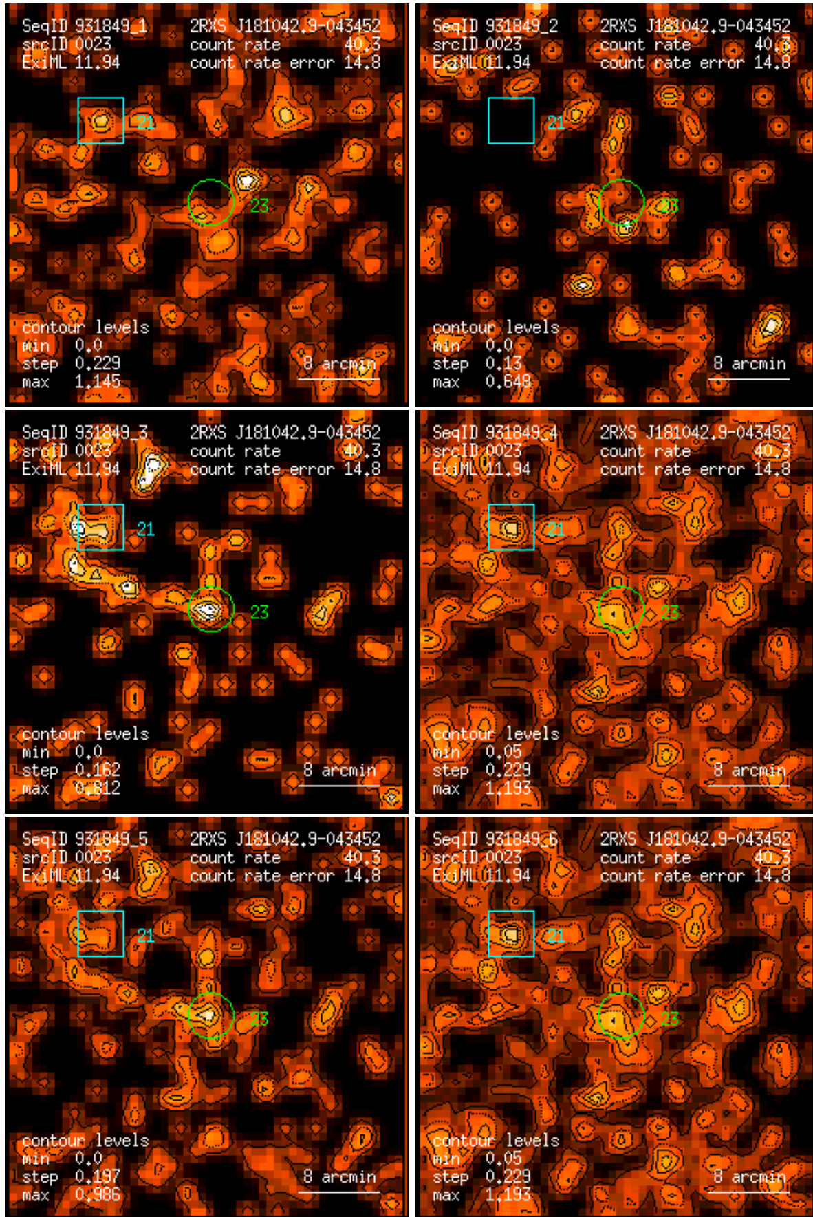
Figure 23: RASS 931849: detection 0023: band rate images, Gaussian filter: (1) PSPC channels 11 – 41, (2) 52 – 90, (3) 91 – 201, (4) 11 – 235, (5) 52 – 201, (6) 11 – 201. Broad band rates in counts/ks. Band rate contour levels in counts/ks/arcmin 2 .
