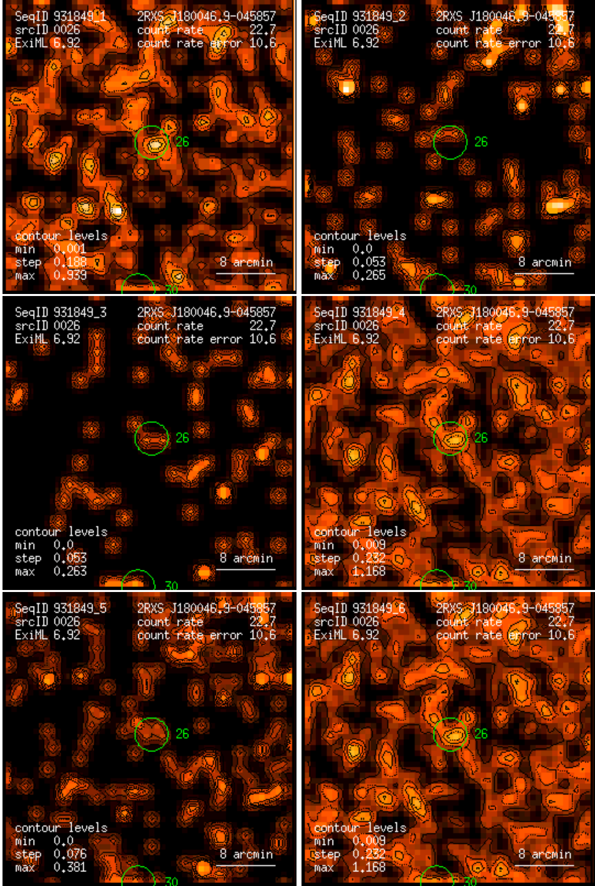
Figure 26: RASS 931849: detection 0026: band rate images, Gaussian filter: (1) PSPC channels 11 – 41, (2) 52 – 90, (3) 91 – 201, (4) 11 – 235, (5) 52 – 201, (6) 11 – 201. Broad band rates in counts/ks. Band rate contour levels in counts/ks/arcmin 2 .
