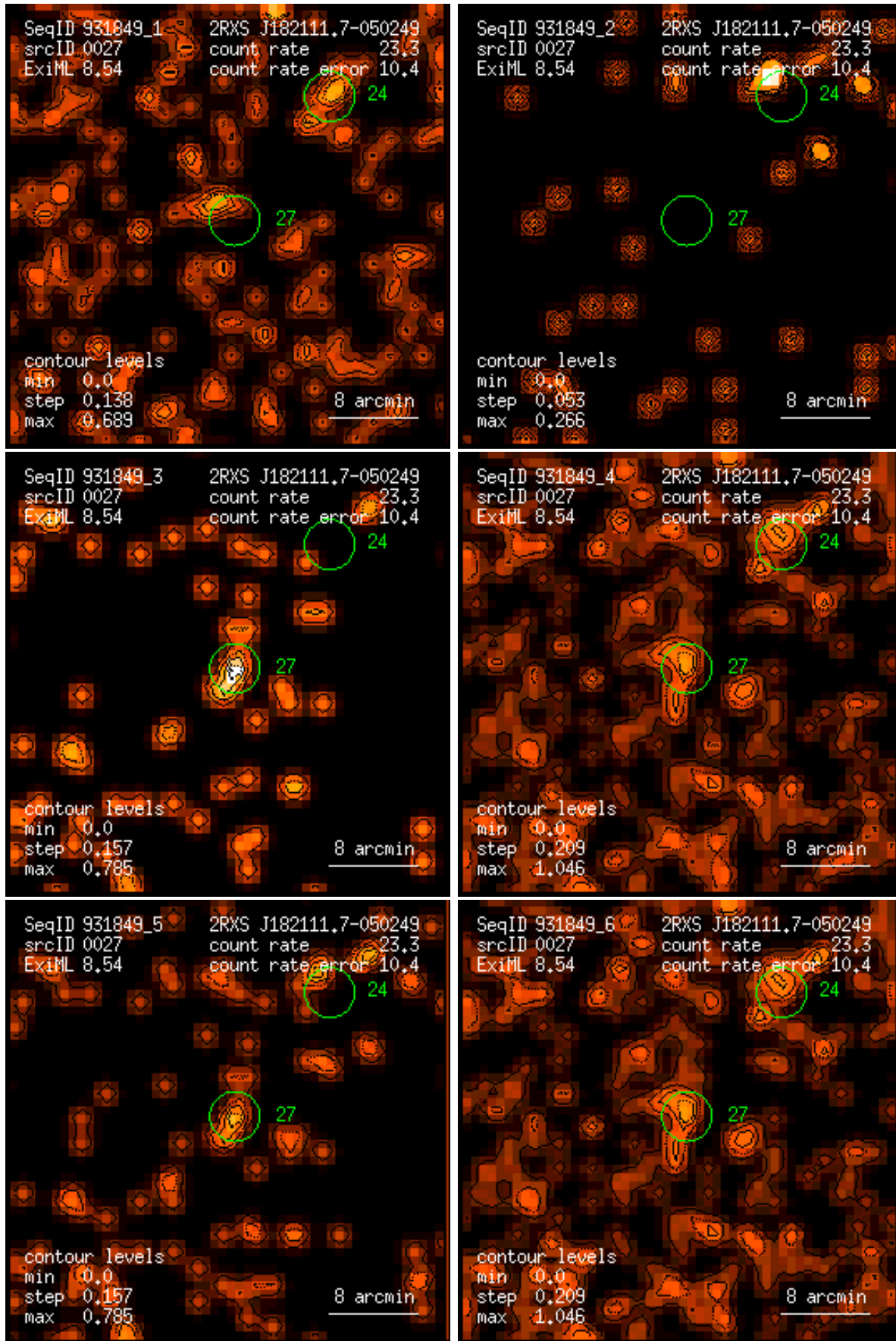
Figure 27: RASS 931849: detection 0027: band rate images, Gaussian filter: (1) PSPC channels 11 – 41, (2) 52 – 90, (3) 91 – 201, (4) 11 – 235, (5) 52 – 201, (6) 11 – 201. Broad band rates in counts/ks. Band rate contour levels in counts/ks/arcmin 2 .
