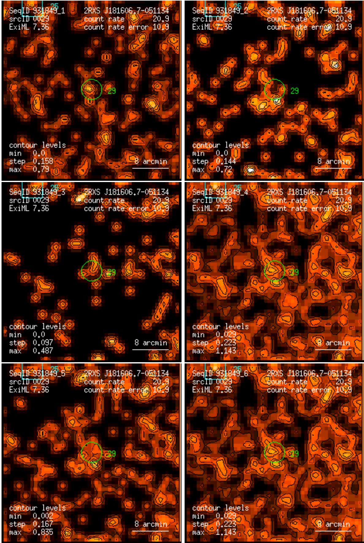
Figure 29: RASS 931849: detection 0029: band rate images, Gaussian filter: (1) PSPC channels 11 – 41, (2) 52 – 90, (3) 91 – 201, (4) 11 – 235, (5) 52 – 201, (6) 11 – 201. Broad band rates in counts/ks. Band rate contour levels in counts/ks/arcmin 2 .
