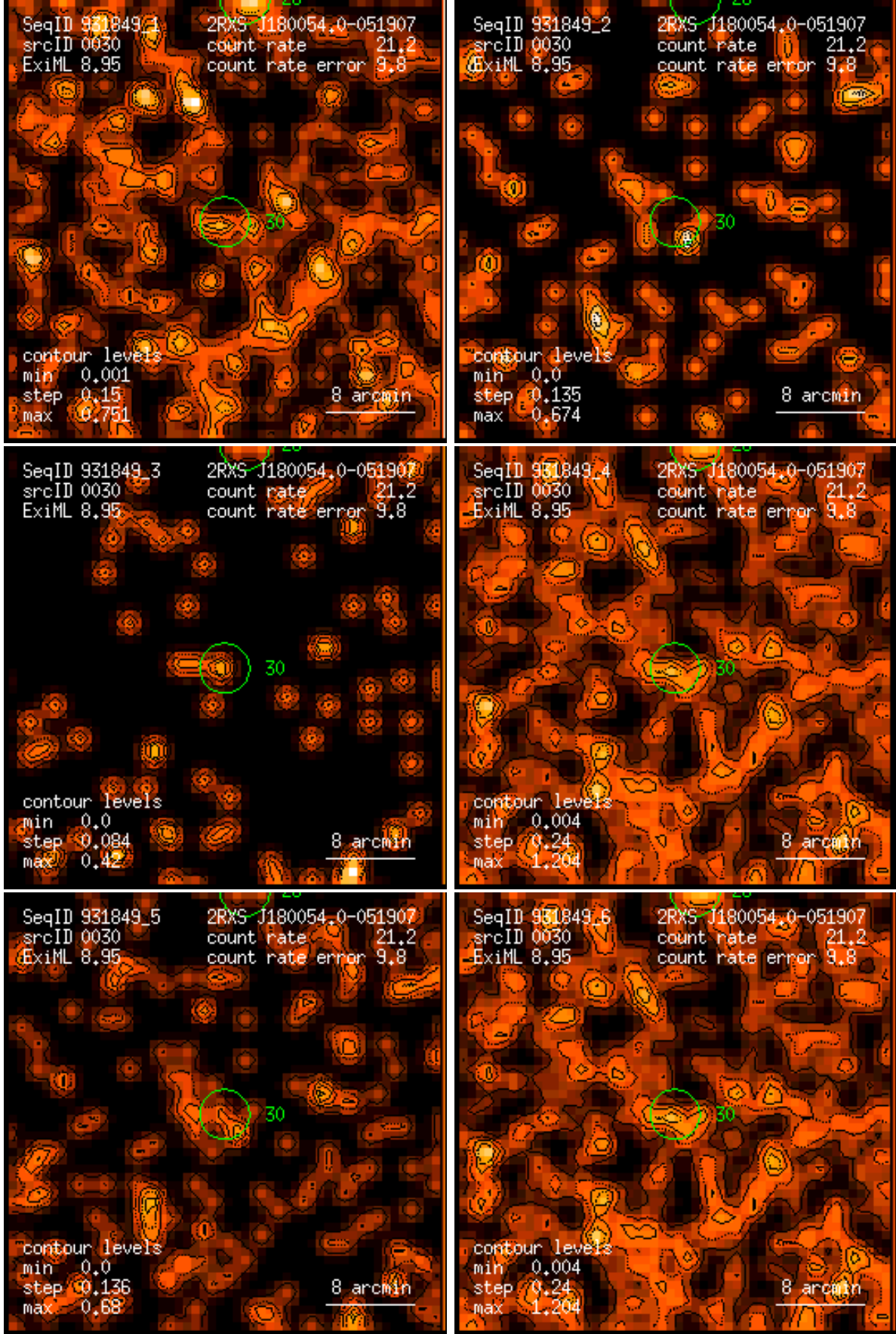
Figure 30: RASS 931849: detection 0030: band rate images, Gaussian filter: (1) PSPC channels 11 – 41, (2) 52 – 90, (3) 91 – 201, (4) 11 – 235, (5) 52 – 201, (6) 11 – 201. Broad band rates in counts/ks. Band rate contour levels in counts/ks/arcmin 2 .
