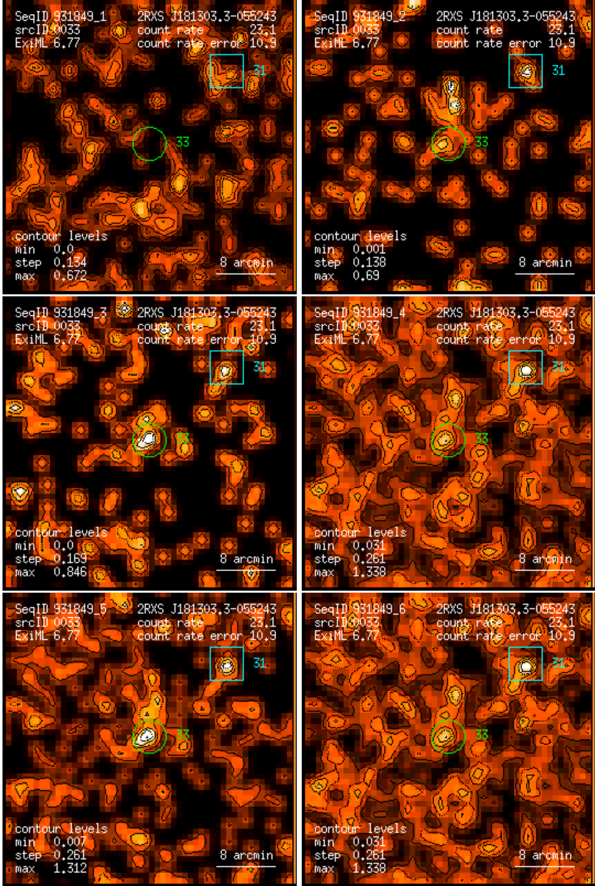
Figure 33: RASS 931849: detection 0033: band rate images, Gaussian filter: (1) PSPC channels 11 – 41, (2) 52 – 90, (3) 91 – 201, (4) 11 – 235, (5) 52 – 201, (6) 11 – 201. Broad band rates in counts/ks. Band rate contour levels in counts/ks/arcmin 2 .
