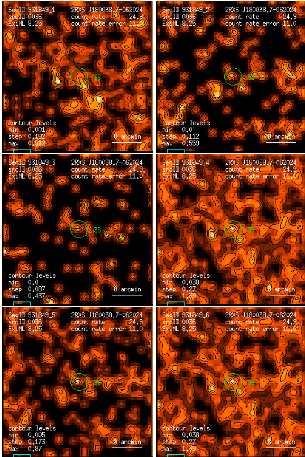
Figure 36: RASS 931849: detection 0036: band rate images, Gaussian filter: (1) PSPC channels 11 – 41, (2) 52 – 90, (3) 91 – 201, (4) 11 – 235, (5) 52 – 201, (6) 11 – 201. Broad band rates in counts/ks. Band rate contour levels in counts/ks/arcmin 2 .
