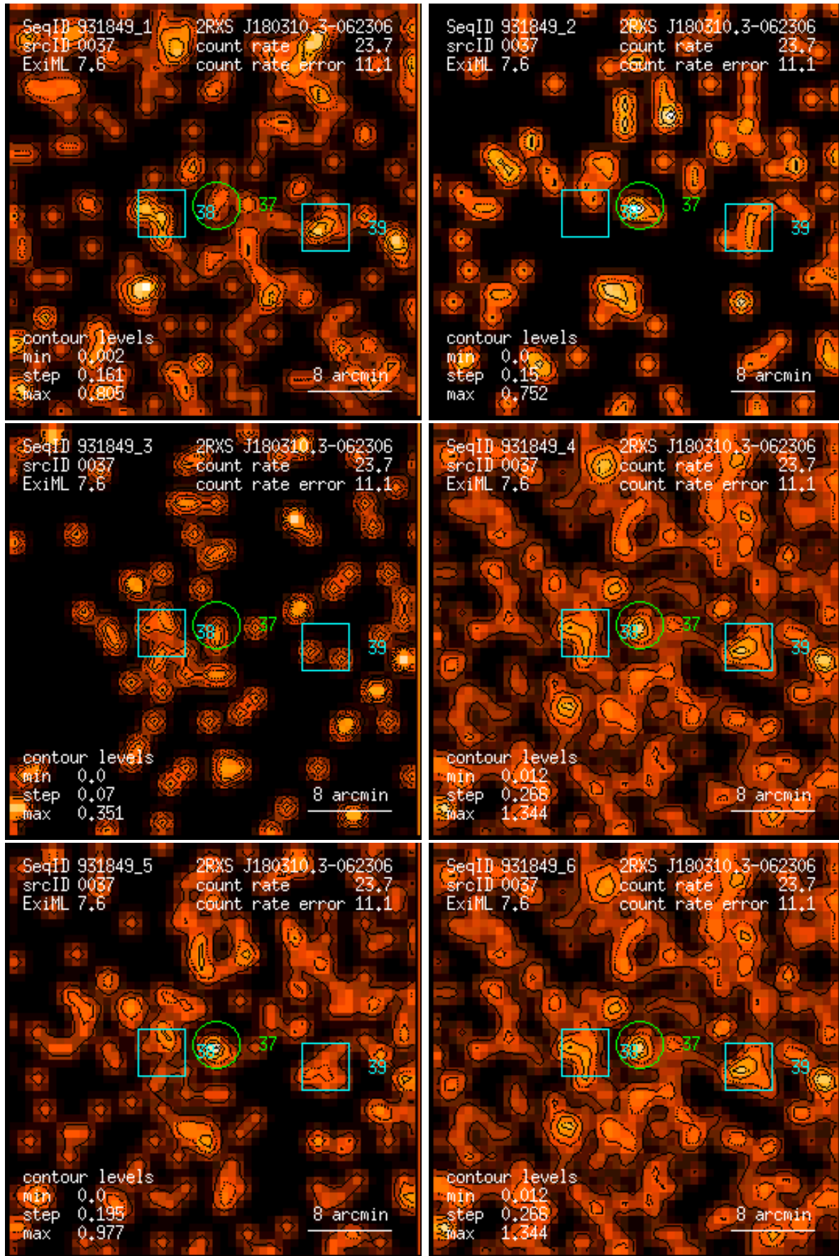
Figure 37: RASS 931849: detection 0037: band rate images, Gaussian filter: (1) PSPC channels 11 – 41, (2) 52 – 90, (3) 91 – 201, (4) 11 – 235, (5) 52 – 201, (6) 11 – 201. Broad band rates in counts/ks. Band rate contour levels in counts/ks/arcmin 2 .
