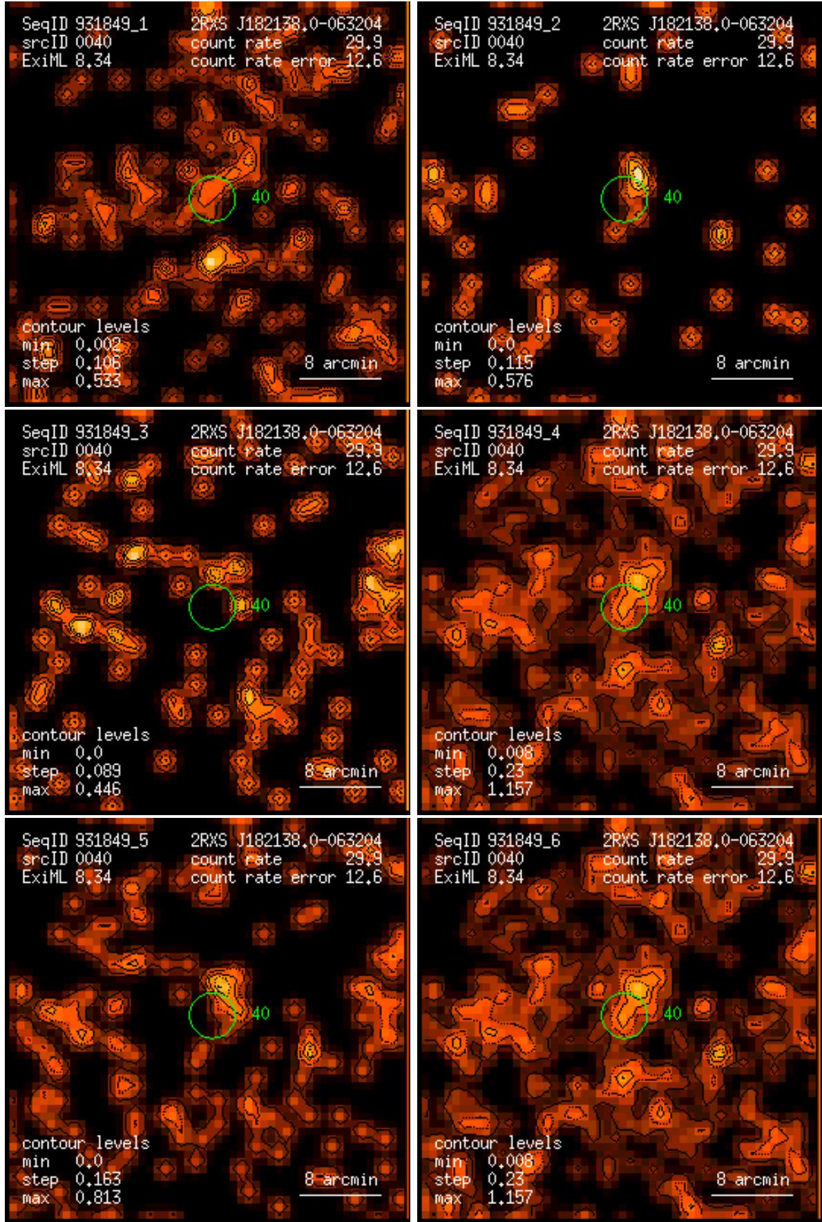
Figure 40: RASS 931849: detection 0040: band rate images, Gaussian filter: (1) PSPC channels 11 – 41, (2) 52 – 90, (3) 91 – 201, (4) 11 – 235, (5) 52 – 201, (6) 11 – 201. Broad band rates in counts/ks. Band rate contour levels in counts/ks/arcmin 2 .
