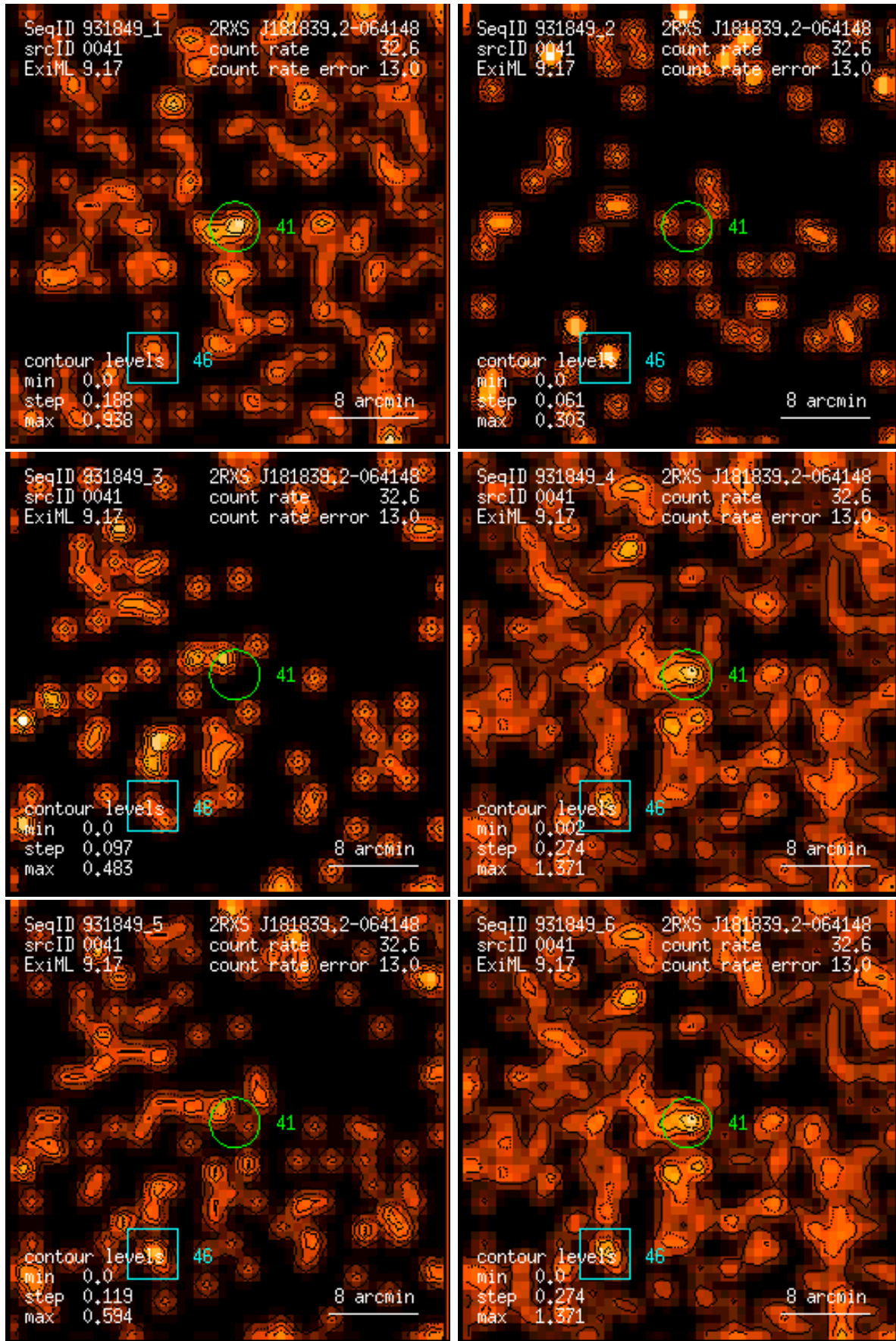
Figure 41: RASS 931849: detection 0041: band rate images, Gaussian filter: (1) PSPC channels 11 – 41, (2) 52 – 90, (3) 91 – 201, (4) 11 – 235, (5) 52 – 201, (6) 11 – 201. Broad band rates in counts/ks. Band rate contour levels in counts/ks/arcmin 2 .
