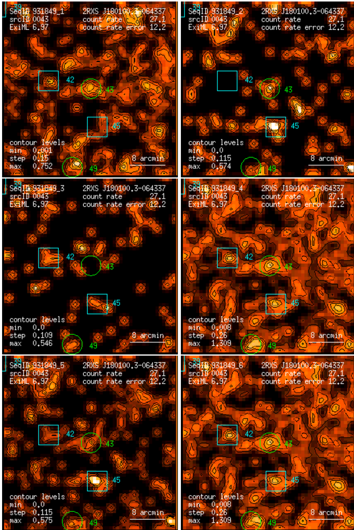
Figure 43: RASS 931849: detection 0043: band rate images, Gaussian filter: (1) PSPC channels 11 – 41, (2) 52 – 90, (3) 91 – 201, (4) 11 – 235, (5) 52 – 201, (6) 11 – 201. Broad band rates in counts/ks. Band rate contour levels in counts/ks/arcmin 2 .
