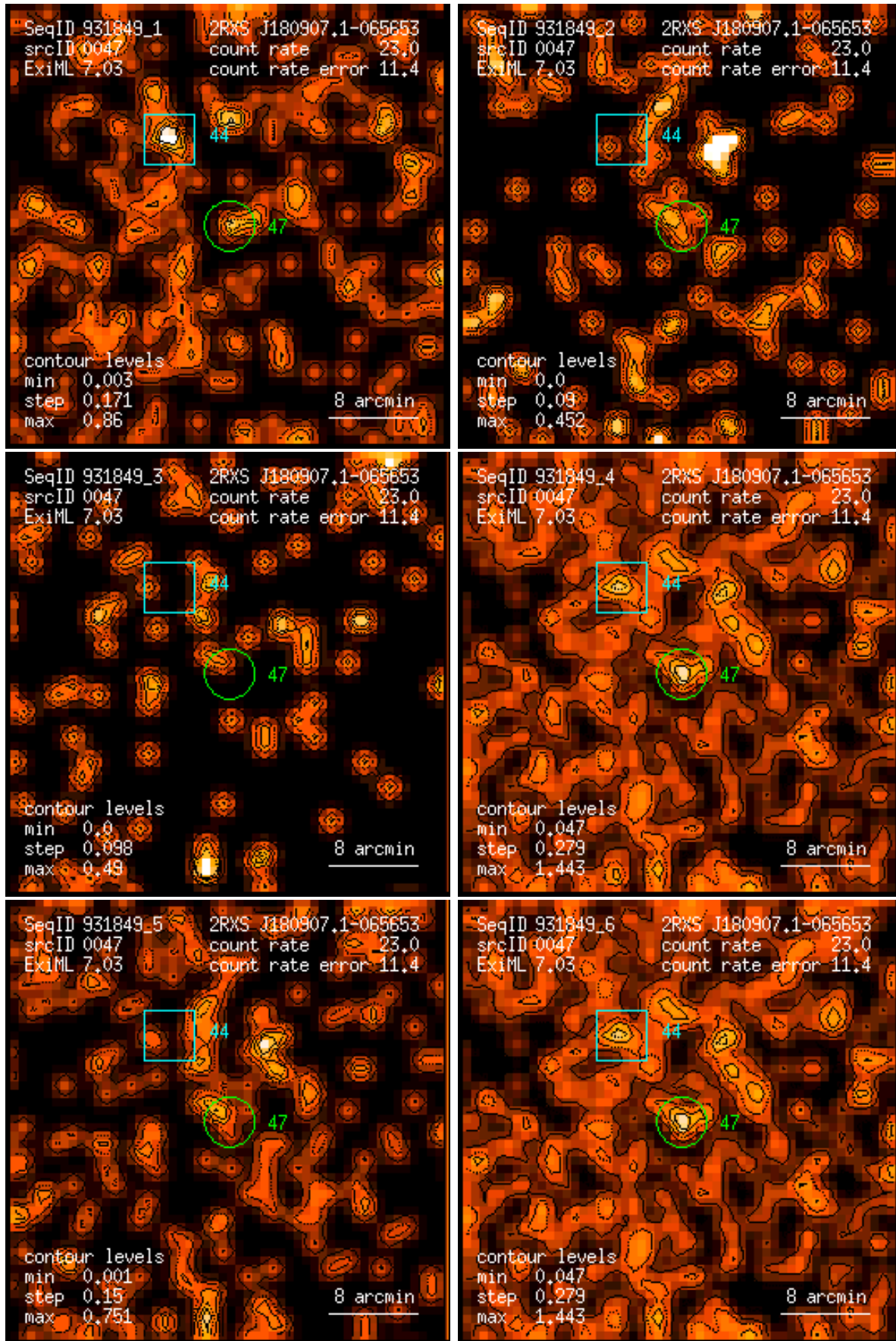
Figure 47: RASS 931849: detection 0047: band rate images, Gaussian filter: (1) PSPC channels 11 – 41, (2) 52 – 90, (3) 91 – 201, (4) 11 – 235, (5) 52 – 201, (6) 11 – 201. Broad band rates in counts/ks. Band rate contour levels in counts/ks/arcmin 2 .
