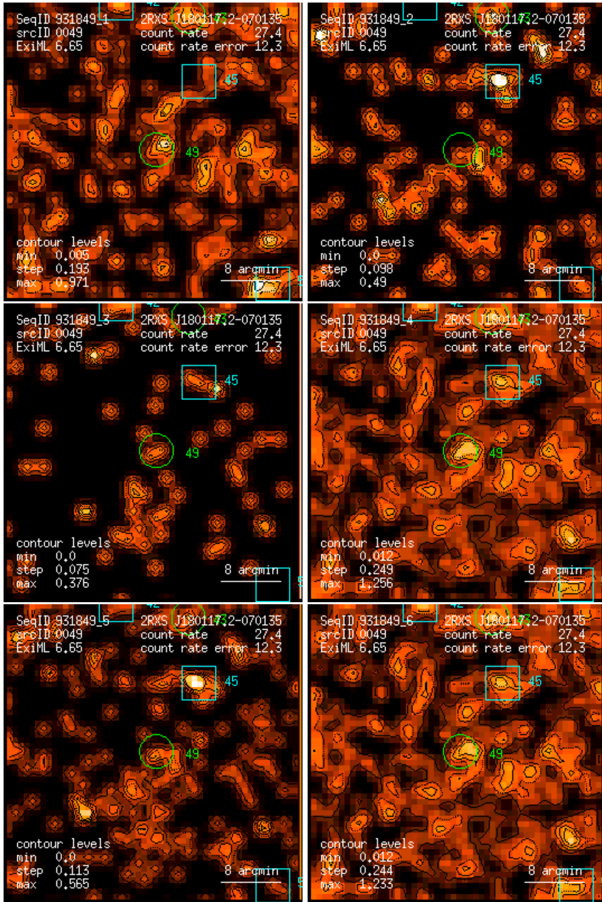
Figure 49: RASS 931849: detection 0049: band rate images, Gaussian filter: (1) PSPC channels 11 – 41, (2) 52 – 90, (3) 91 – 201, (4) 11 – 235, (5) 52 – 201, (6) 11 – 201. Broad band rates in counts/ks. Band rate contour levels in counts/ks/arcmin 2 .
