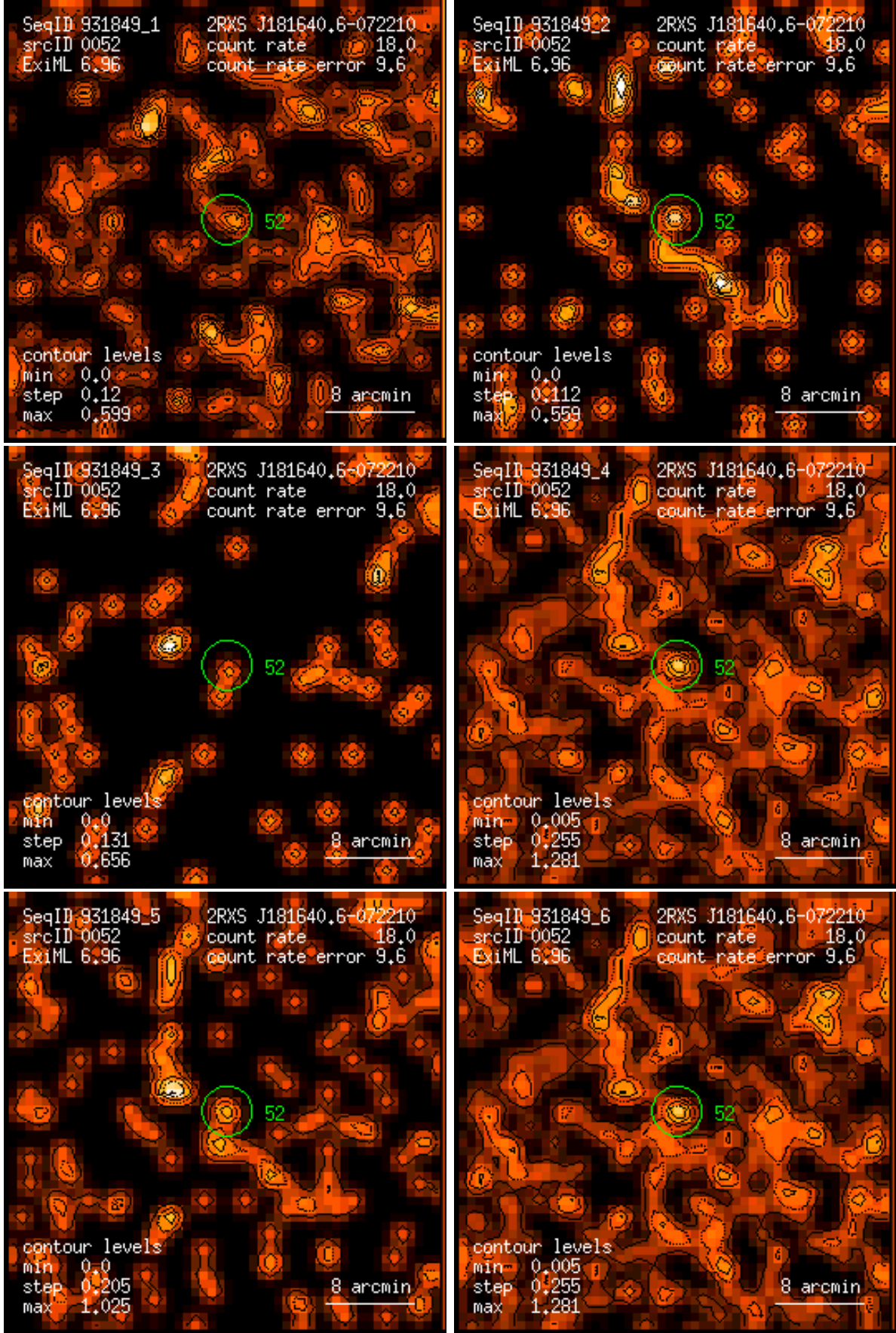
Figure 52: RASS 931849: detection 0052: band rate images, Gaussian filter: (1) PSPC channels 11 – 41, (2) 52 – 90, (3) 91 – 201, (4) 11 – 235, (5) 52 – 201, (6) 11 – 201. Broad band rates in counts/ks. Band rate contour levels in counts/ks/arcmin 2 .
