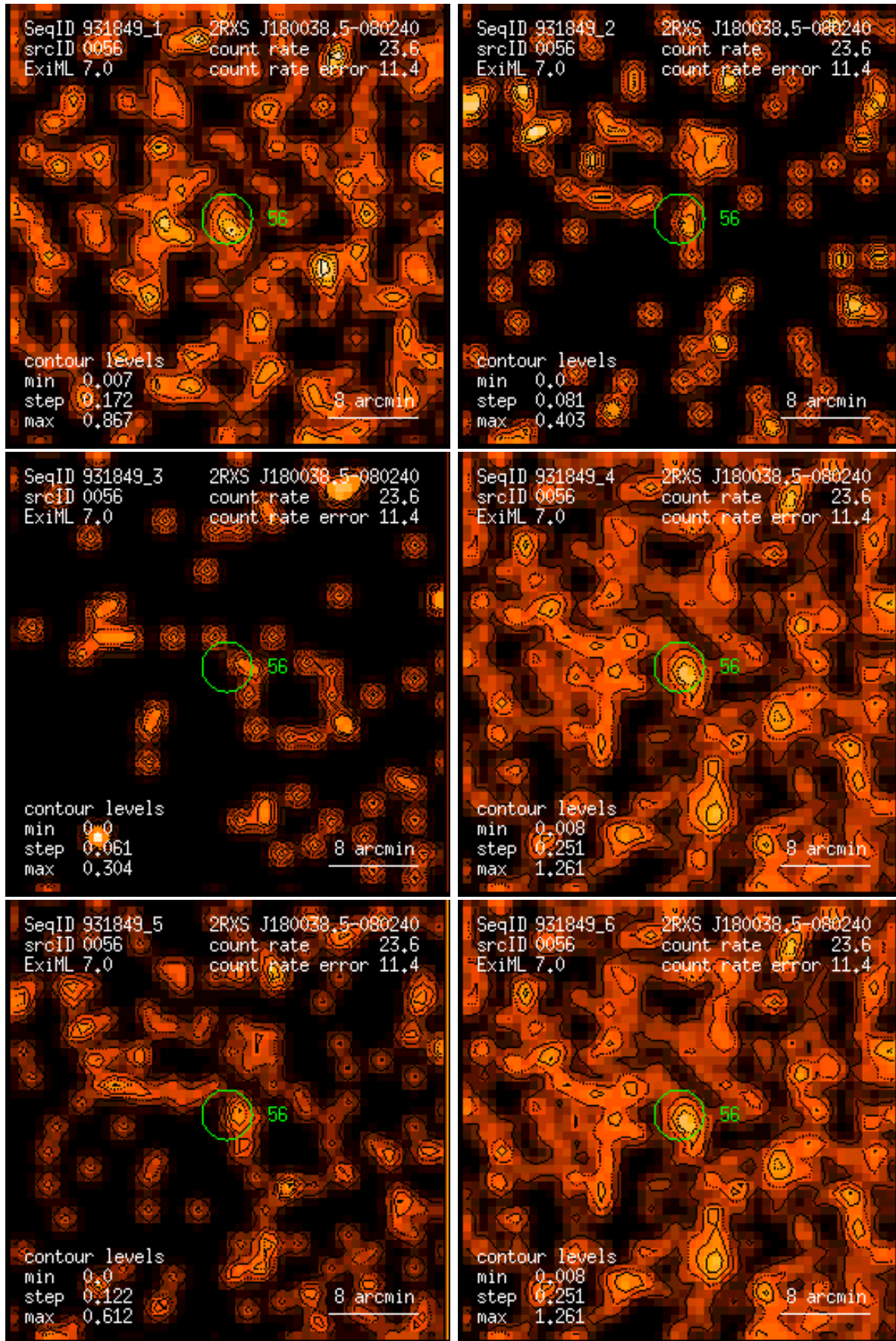
Figure 56: RASS 931849: detection 0056: band rate images, Gaussian filter: (1) PSPC channels 11 – 41, (2) 52 – 90, (3) 91 – 201, (4) 11 – 235, (5) 52 – 201, (6) 11 – 201. Broad band rates in counts/ks. Band rate contour levels in counts/ks/arcmin 2 .
