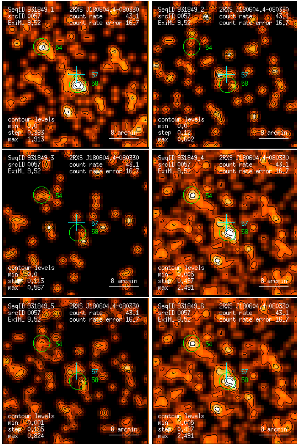
Figure 57: RASS 931849: detection 0057: band rate images, Gaussian filter: (1) PSPC channels 11 – 41, (2) 52 – 90, (3) 91 – 201, (4) 11 – 235, (5) 52 – 201, (6) 11 – 201. Broad band rates in counts/ks. Band rate contour levels in counts/ks/arcmin 2 .
