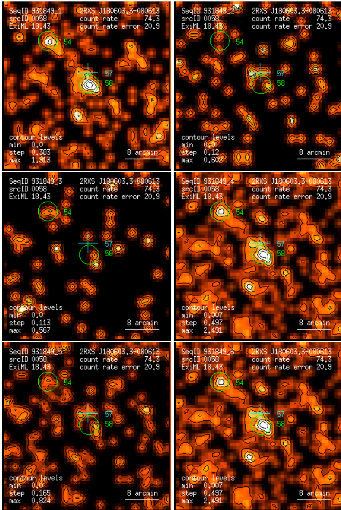
Figure 58: RASS 931849: detection 0058: band rate images, Gaussian filter: (1) PSPC channels 11 – 41, (2) 52 – 90, (3) 91 – 201, (4) 11 – 235, (5) 52 – 201, (6) 11 – 201. Broad band rates in counts/ks. Band rate contour levels in counts/ks/arcmin 2 .
