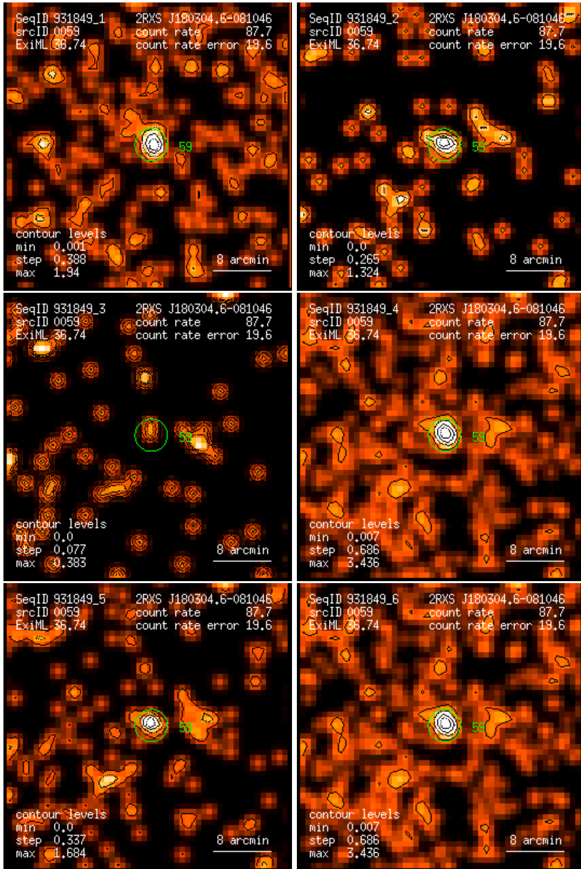
Figure 59: RASS 931849: detection 0059: band rate images, Gaussian filter: (1) PSPC channels 11 – 41, (2) 52 – 90, (3) 91 – 201, (4) 11 – 235, (5) 52 – 201, (6) 11 – 201. Broad band rates in counts/ks. Band rate contour levels in counts/ks/arcmin 2 .
