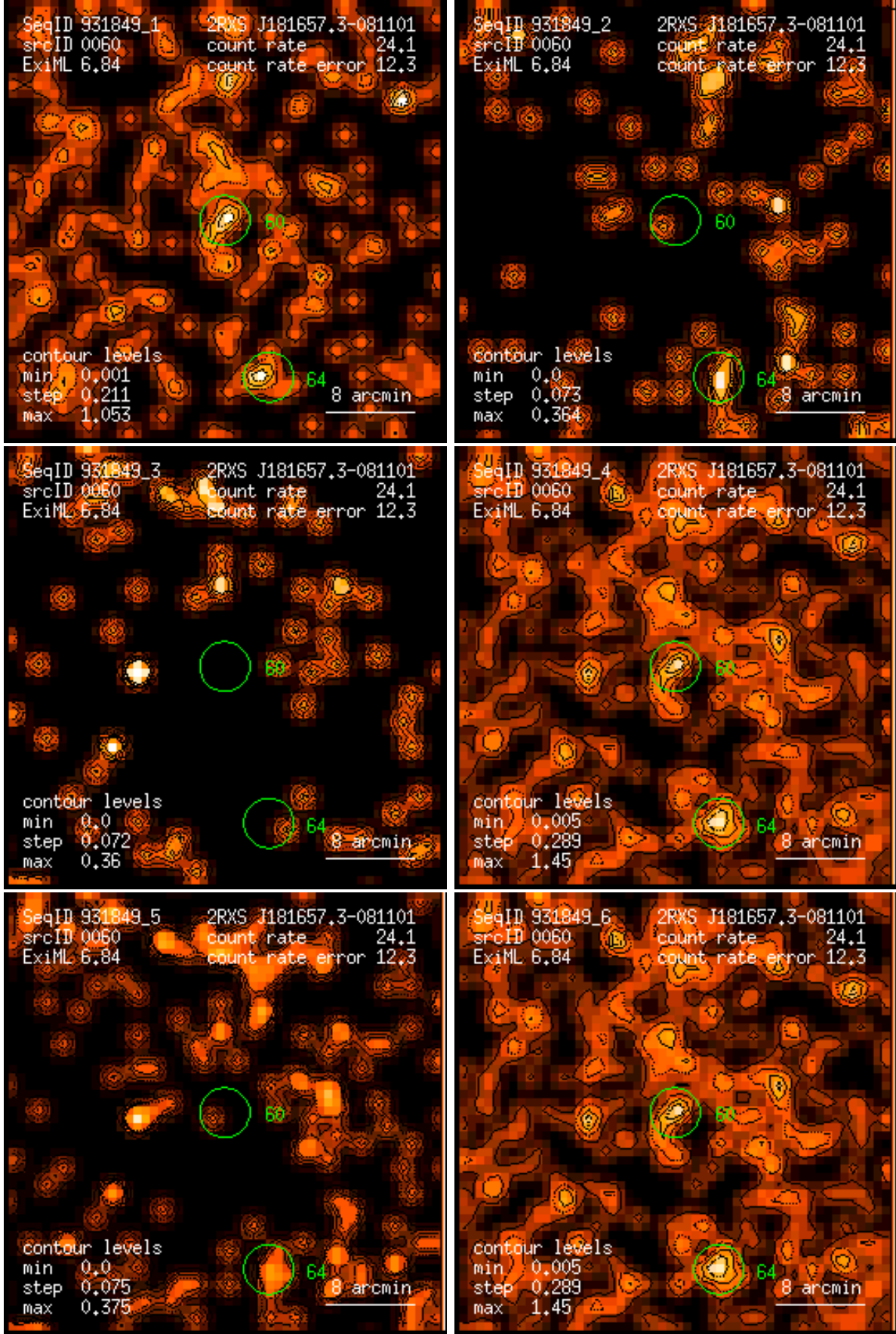
Figure 60: RASS 931849: detection 0060: band rate images, Gaussian filter: (1) PSPC channels 11 – 41, (2) 52 – 90, (3) 91 – 201, (4) 11 – 235, (5) 52 – 201, (6) 11 – 201. Broad band rates in counts/ks. Band rate contour levels in counts/ks/arcmin 2 .
