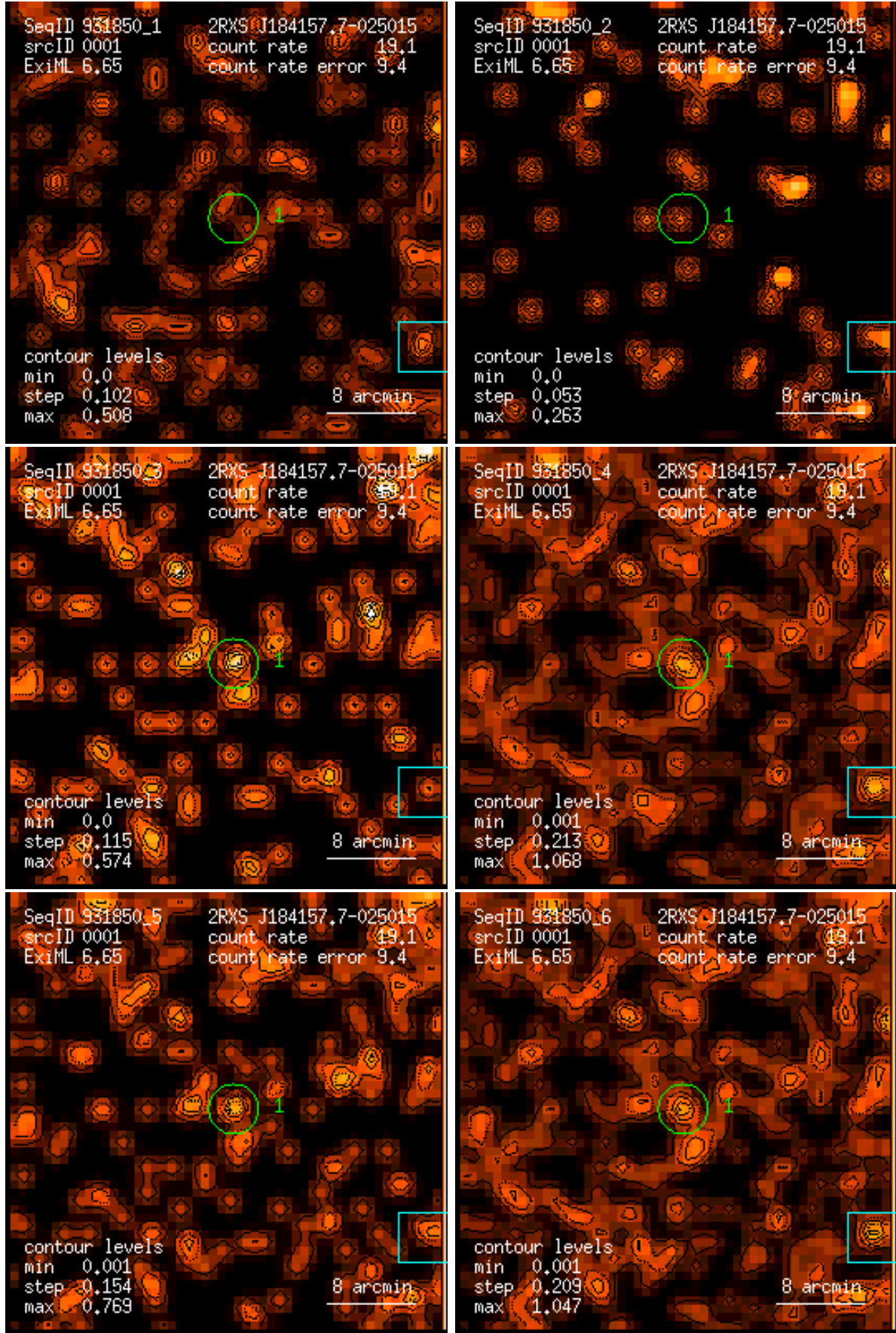
Figure 1: RASS 931850: detection 0001: band rate images, Gaussian filter: (1) PSPC channels 11 – 41, (2) 52 – 90, (3) 91 – 201, (4) 11 – 235, (5) 52 – 201, (6) 11 – 201. Broad band rates in counts/ks. Band rate contour levels in counts/ks/arcmin 2 .
