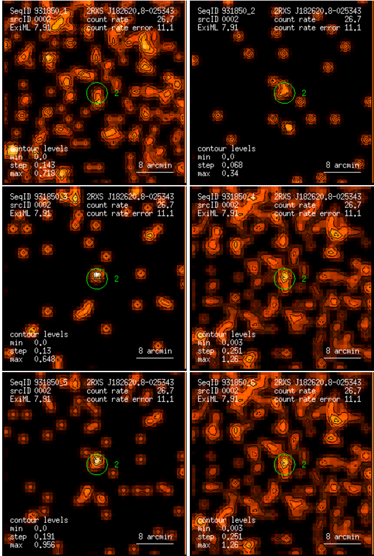
Figure 2: RASS 931850: detection 0002: band rate images, Gaussian filter: (1) PSPC channels 11 – 41, (2) 52 – 90, (3) 91 – 201, (4) 11 – 235, (5) 52 – 201, (6) 11 – 201. Broad band rates in counts/ks. Band rate contour levels in counts/ks/arcmin 2 .
