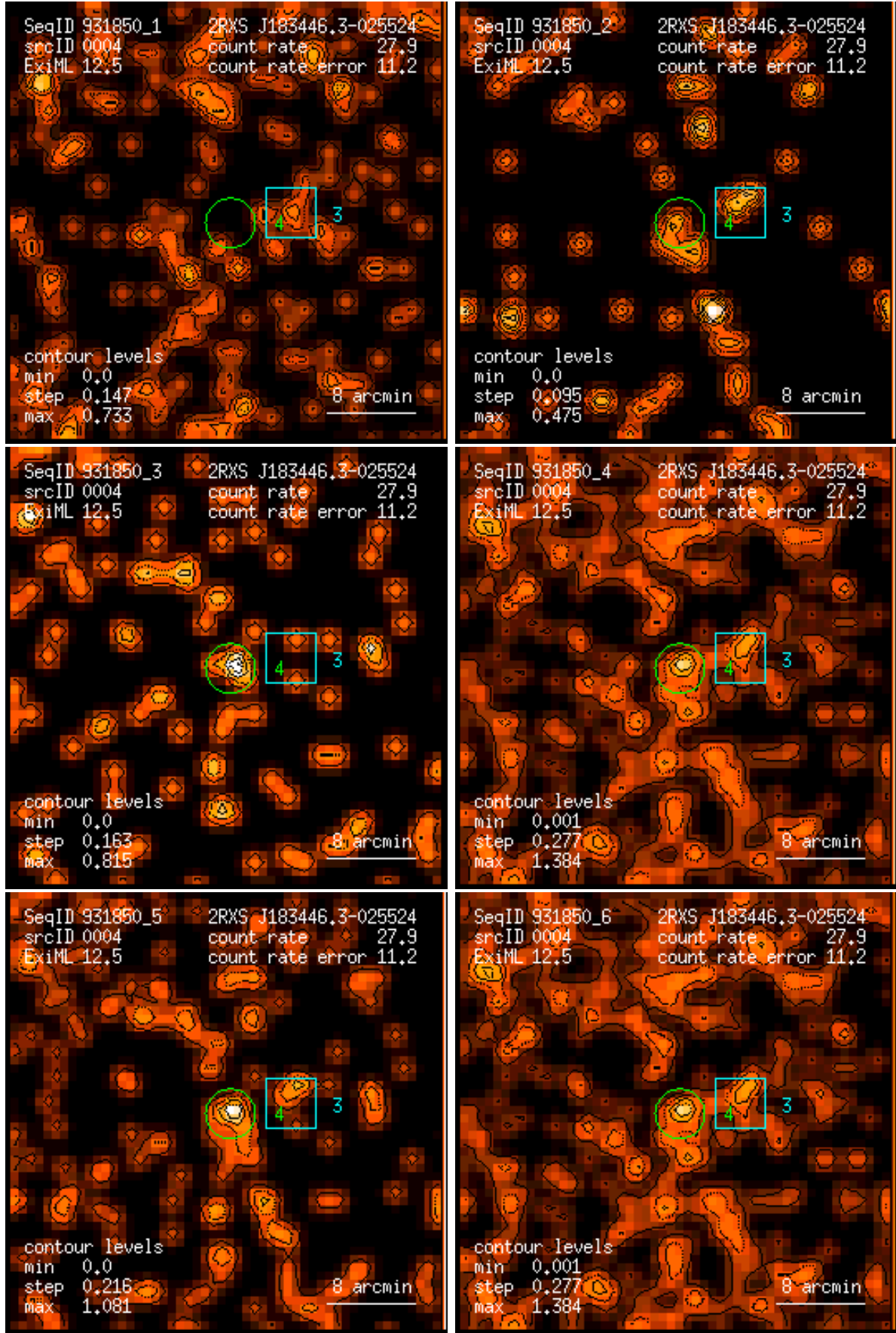
Figure 4: RASS 931850: detection 0004: band rate images, Gaussian filter: (1) PSPC channels 11 – 41, (2) 52 – 90, (3) 91 – 201, (4) 11 – 235, (5) 52 – 201, (6) 11 – 201. Broad band rates in counts/ks. Band rate contour levels in counts/ks/arcmin 2 .
