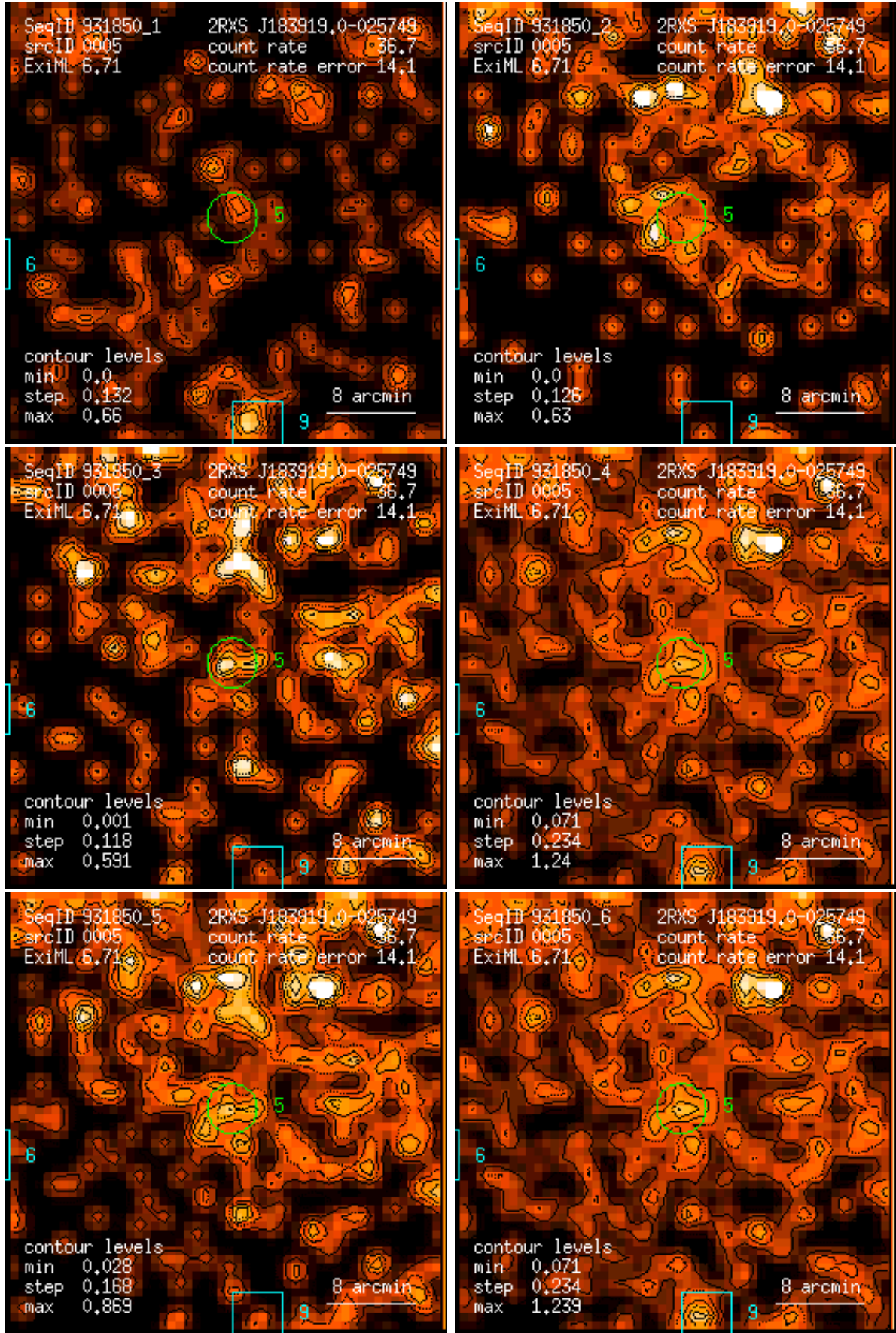
Figure 5: RASS 931850: detection 0005: band rate images, Gaussian filter: (1) PSPC channels 11 – 41, (2) 52 – 90, (3) 91 – 201, (4) 11 – 235, (5) 52 – 201, (6) 11 – 201. Broad band rates in counts/ks. Band rate contour levels in counts/ks/arcmin 2 .
