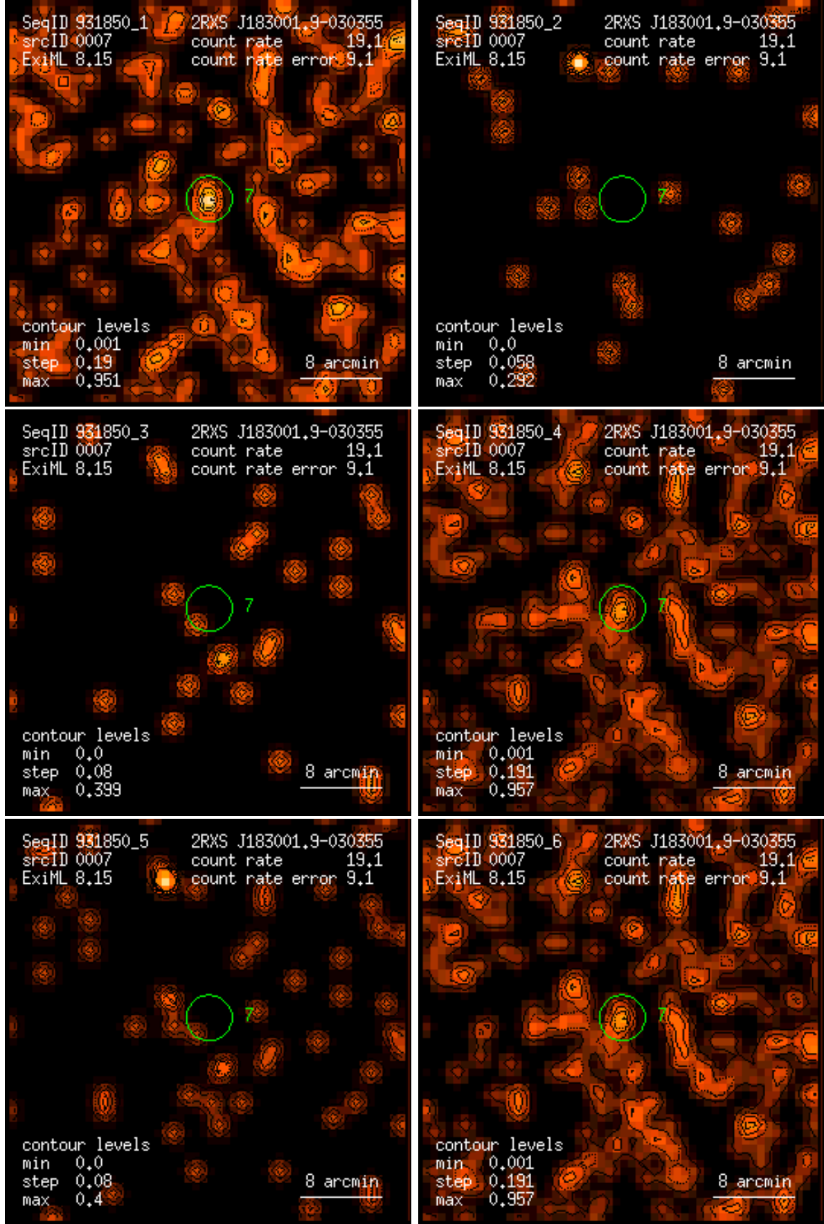
Figure 7: RASS 931850: detection 0007: band rate images, Gaussian filter: (1) PSPC channels 11 – 41, (2) 52 – 90, (3) 91 – 201, (4) 11 – 235, (5) 52 – 201, (6) 11 – 201. Broad band rates in counts/ks. Band rate contour levels in counts/ks/arcmin 2 .
