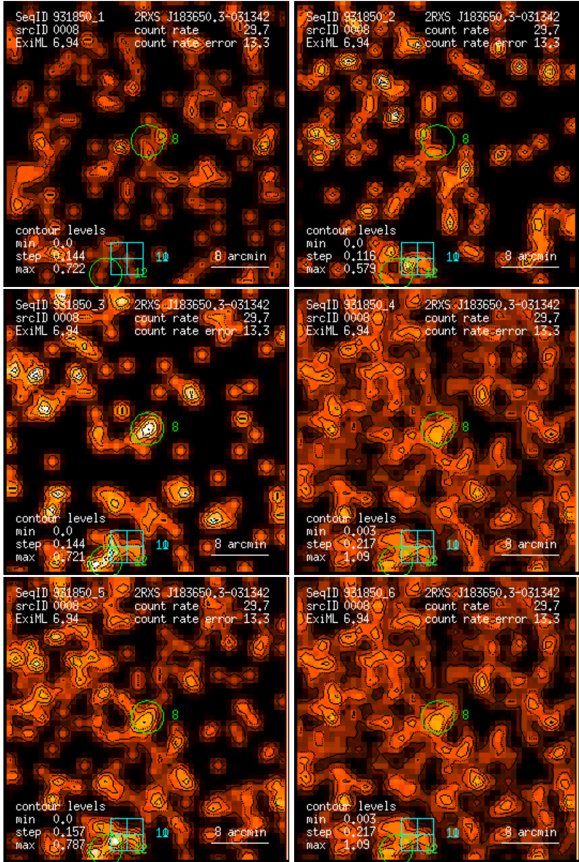
Figure 8: RASS 931850: detection 0008: band rate images, Gaussian filter: (1) PSPC channels 11 – 41, (2) 52 – 90, (3) 91 – 201, (4) 11 – 235, (5) 52 – 201, (6) 11 – 201. Broad band rates in counts/ks. Band rate contour levels in counts/ks/arcmin 2 .
