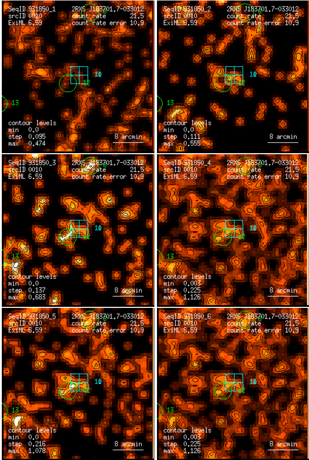
Figure 10: RASS 931850: detection 0010: band rate images, Gaussian filter: (1) PSPC channels 11 – 41, (2) 52 – 90, (3) 91 – 201, (4) 11 – 235, (5) 52 – 201, (6) 11 – 201. Broad band rates in counts/ks. Band rate contour levels in counts/ks/arcmin 2 .
