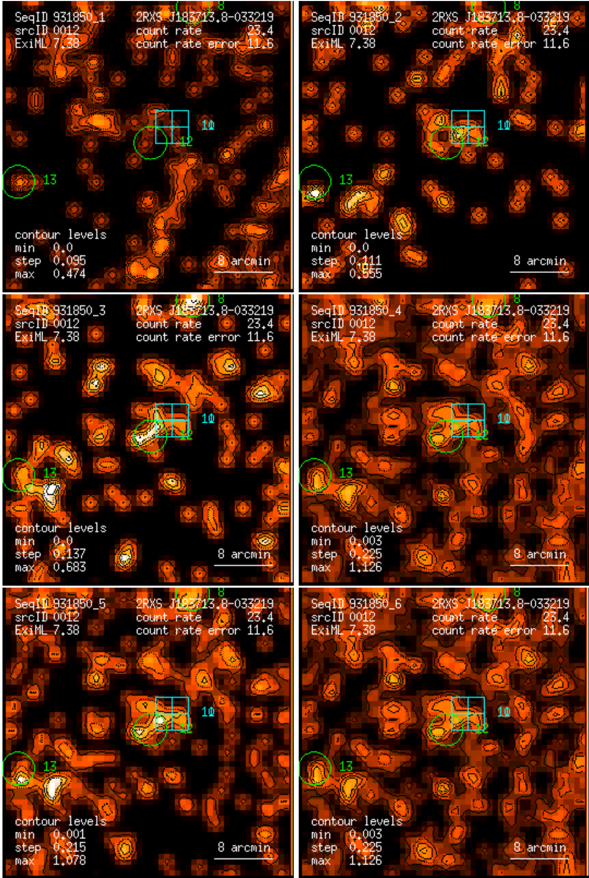
Figure 12: RASS 931850: detection 0012: band rate images, Gaussian filter: (1) PSPC channels 11 – 41, (2) 52 – 90, (3) 91 – 201, (4) 11 – 235, (5) 52 – 201, (6) 11 – 201. Broad band rates in counts/ks. Band rate contour levels in counts/ks/arcmin 2 .
