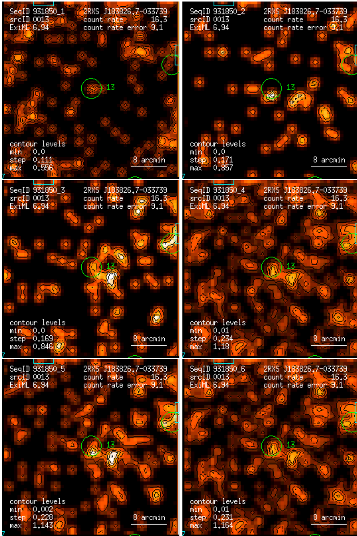
Figure 13: RASS 931850: detection 0013: band rate images, Gaussian filter: (1) PSPC channels 11 – 41, (2) 52 – 90, (3) 91 – 201, (4) 11 – 235, (5) 52 – 201, (6) 11 – 201. Broad band rates in counts/ks. Band rate contour levels in counts/ks/arcmin 2 .
