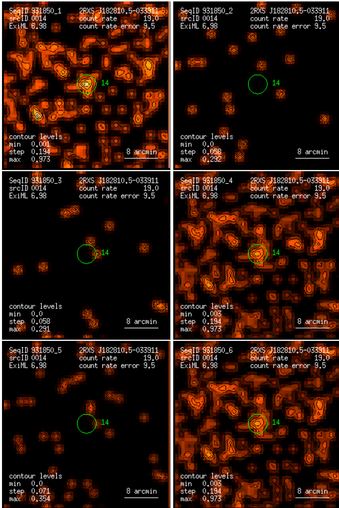
Figure 14: RASS 931850: detection 0014: band rate images, Gaussian filter: (1) PSPC channels 11 – 41, (2) 52 – 90, (3) 91 – 201, (4) 11 – 235, (5) 52 – 201, (6) 11 – 201. Broad band rates in counts/ks. Band rate contour levels in counts/ks/arcmin 2 .
