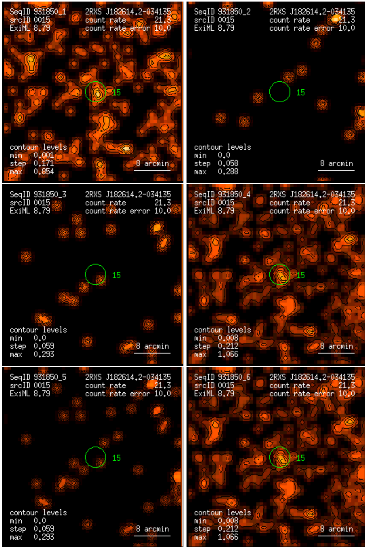
Figure 15: RASS 931850: detection 0015: band rate images, Gaussian filter: (1) PSPC channels 11 – 41, (2) 52 – 90, (3) 91 – 201, (4) 11 – 235, (5) 52 – 201, (6) 11 – 201. Broad band rates in counts/ks. Band rate contour levels in counts/ks/arcmin 2 .
