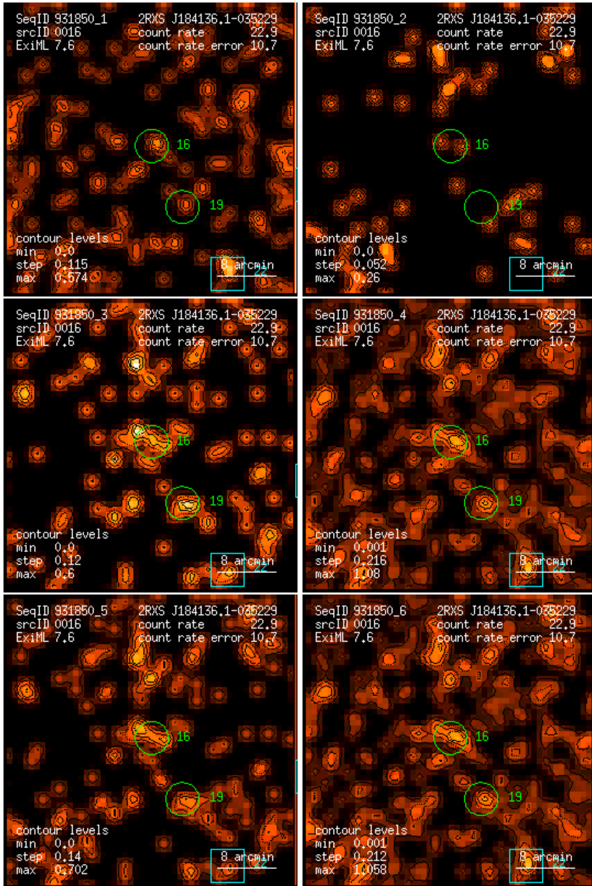
Figure 16: RASS 931850: detection 0016: band rate images, Gaussian filter: (1) PSPC channels 11 – 41, (2) 52 – 90, (3) 91 – 201, (4) 11 – 235, (5) 52 – 201, (6) 11 – 201. Broad band rates in counts/ks. Band rate contour levels in counts/ks/arcmin 2 .
