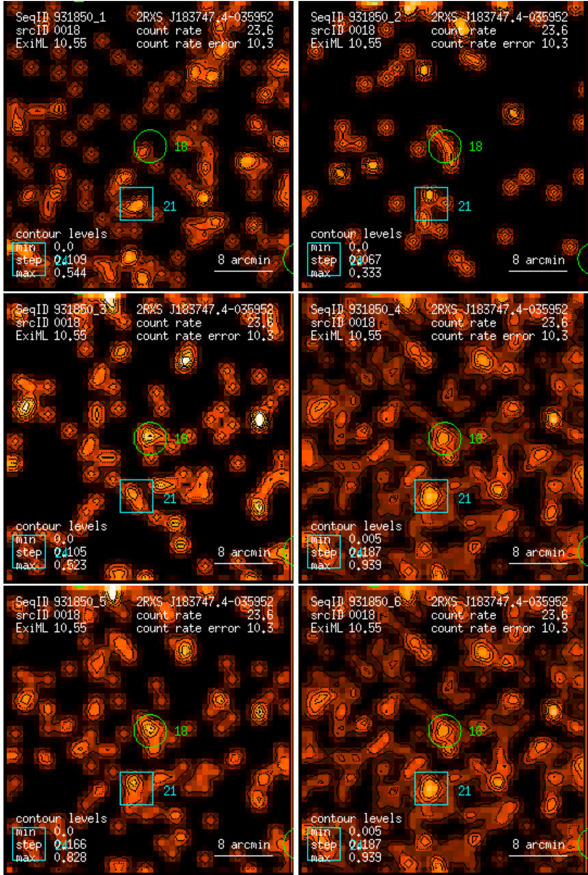
Figure 18: RASS 931850: detection 0018: band rate images, Gaussian filter: (1) PSPC channels 11 – 41, (2) 52 – 90, (3) 91 – 201, (4) 11 – 235, (5) 52 – 201, (6) 11 – 201. Broad band rates in counts/ks. Band rate contour levels in counts/ks/arcmin 2 .
