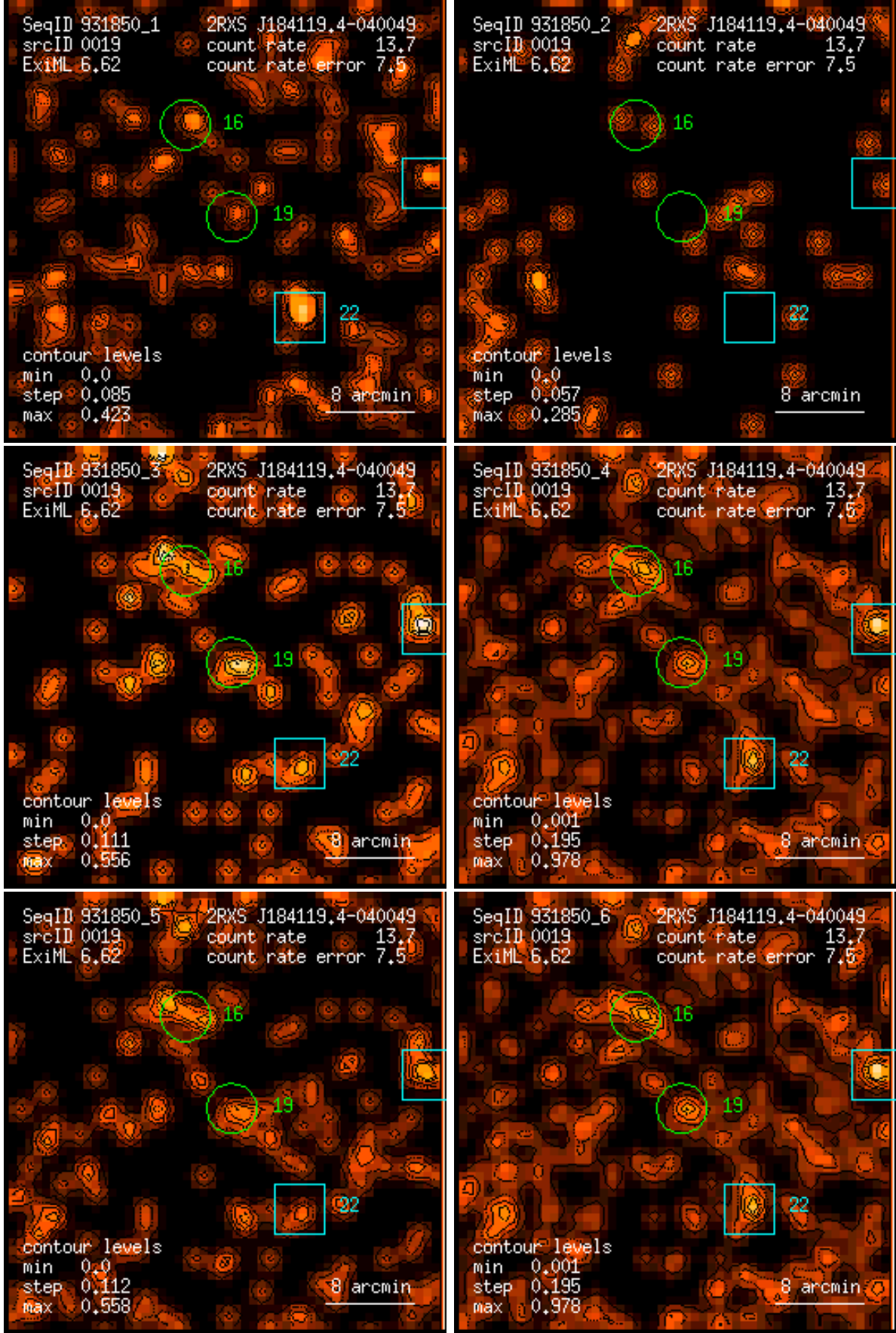
Figure 19: RASS 931850: detection 0019: band rate images, Gaussian filter: (1) PSPC channels 11 – 41, (2) 52 – 90, (3) 91 – 201, (4) 11 – 235, (5) 52 – 201, (6) 11 – 201. Broad band rates in counts/ks. Band rate contour levels in counts/ks/arcmin 2 .
