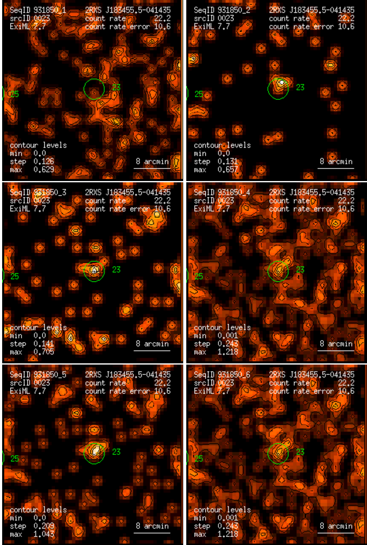
Figure 23: RASS 931850: detection 0023: band rate images, Gaussian filter: (1) PSPC channels 11 – 41, (2) 52 – 90, (3) 91 – 201, (4) 11 – 235, (5) 52 – 201, (6) 11 – 201. Broad band rates in counts/ks. Band rate contour levels in counts/ks/arcmin 2 .
