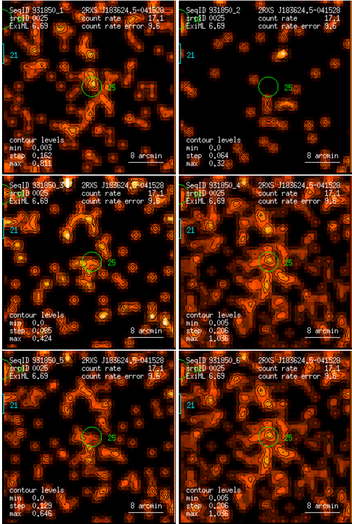
Figure 25: RASS 931850: detection 0025: band rate images, Gaussian filter: (1) PSPC channels 11 – 41, (2) 52 – 90, (3) 91 – 201, (4) 11 – 235, (5) 52 – 201, (6) 11 – 201. Broad band rates in counts/ks. Band rate contour levels in counts/ks/arcmin 2 .
