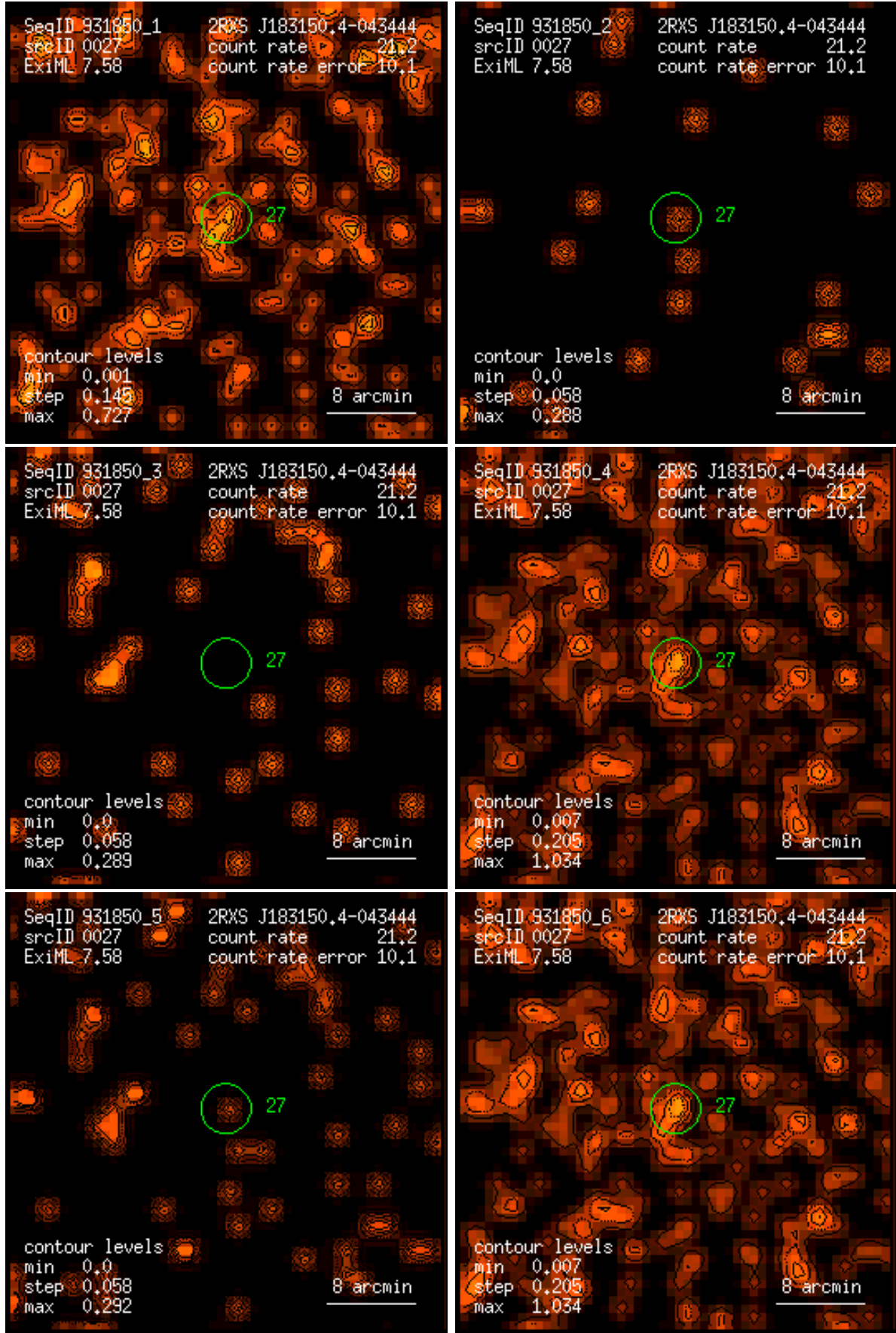
Figure 27: RASS 931850: detection 0027: band rate images, Gaussian filter: (1) PSPC channels 11 – 41, (2) 52 – 90, (3) 91 – 201, (4) 11 – 235, (5) 52 – 201, (6) 11 – 201. Broad band rates in counts/ks. Band rate contour levels in counts/ks/arcmin 2 .
