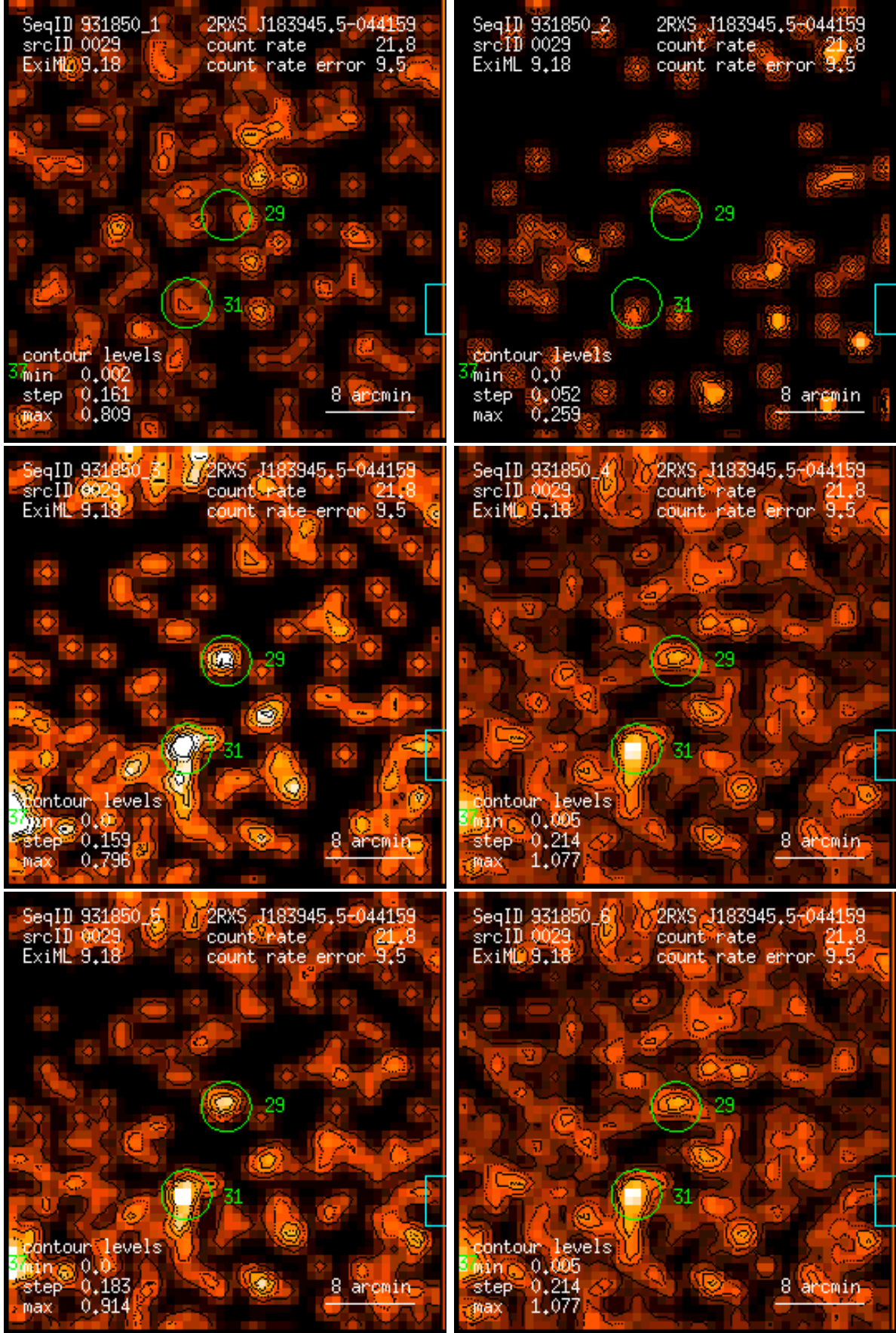
Figure 29: RASS 931850: detection 0029: band rate images, Gaussian filter: (1) PSPC channels 11 – 41, (2) 52 – 90, (3) 91 – 201, (4) 11 – 235, (5) 52 – 201, (6) 11 – 201. Broad band rates in counts/ks. Band rate contour levels in counts/ks/arcmin 2 .
