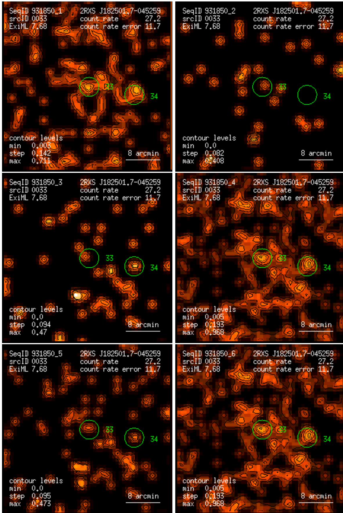
Figure 33: RASS 931850: detection 0033: band rate images, Gaussian filter: (1) PSPC channels 11 – 41, (2) 52 – 90, (3) 91 – 201, (4) 11 – 235, (5) 52 – 201, (6) 11 – 201. Broad band rates in counts/ks. Band rate contour levels in counts/ks/arcmin 2 .
