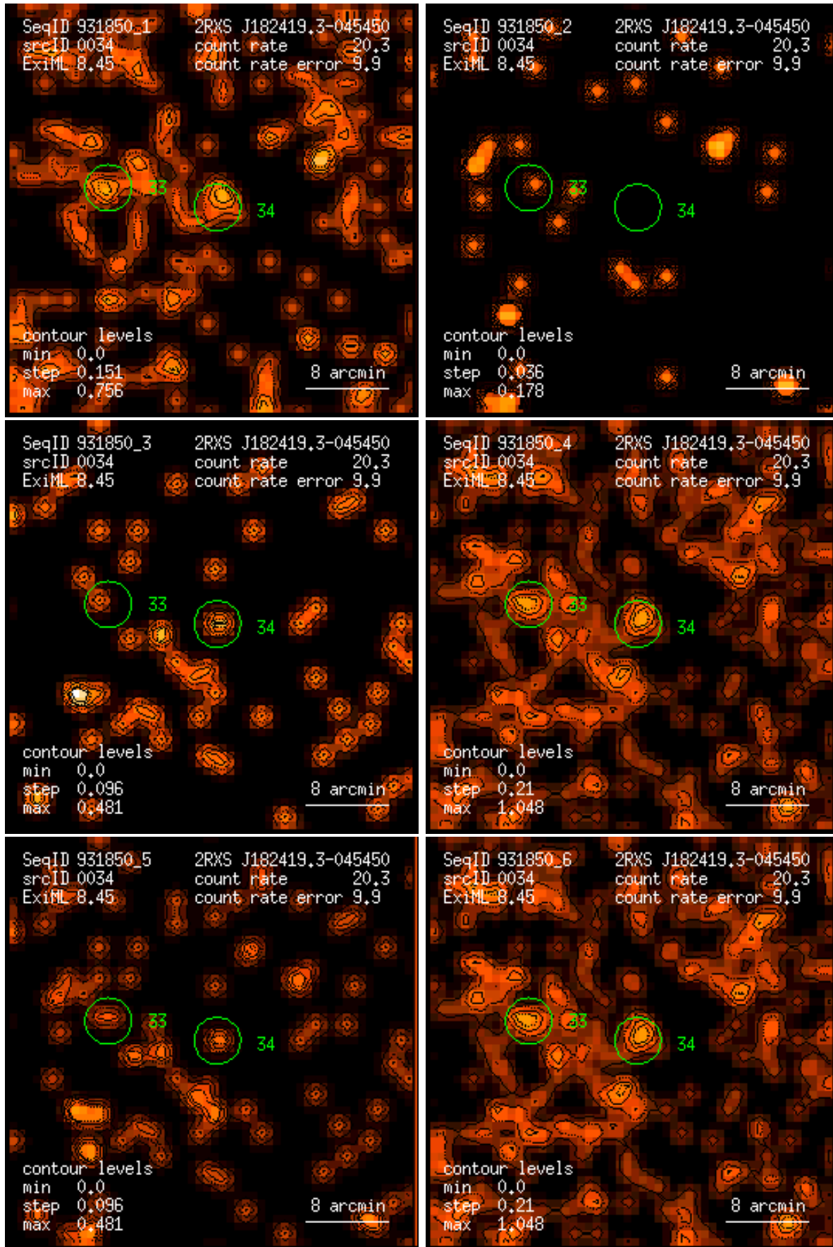
Figure 34: RASS 931850: detection 0034: band rate images, Gaussian filter: (1) PSPC channels 11 – 41, (2) 52 – 90, (3) 91 – 201, (4) 11 – 235, (5) 52 – 201, (6) 11 – 201. Broad band rates in counts/ks. Band rate contour levels in counts/ks/arcmin 2 .
