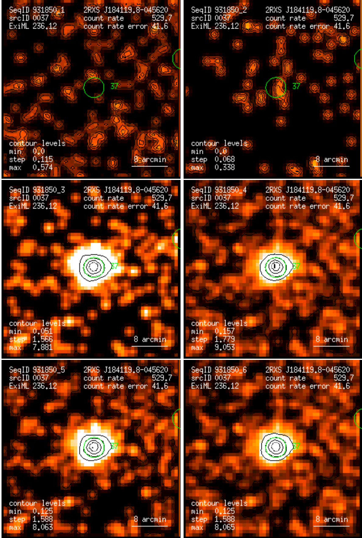
Figure 37: RASS 931850: detection 0037: band rate images, Gaussian filter: (1) PSPC channels 11 – 41, (2) 52 – 90, (3) 91 – 201, (4) 11 – 235, (5) 52 – 201, (6) 11 – 201. Broad band rates in counts/ks. Band rate contour levels in counts/ks/arcmin 2 .
